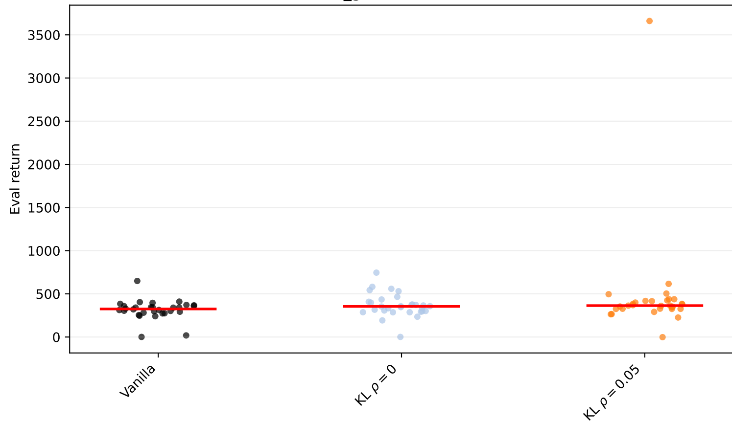
Walker2d-v5 actuator_gain factor=0.5: seed scatter (raw)
