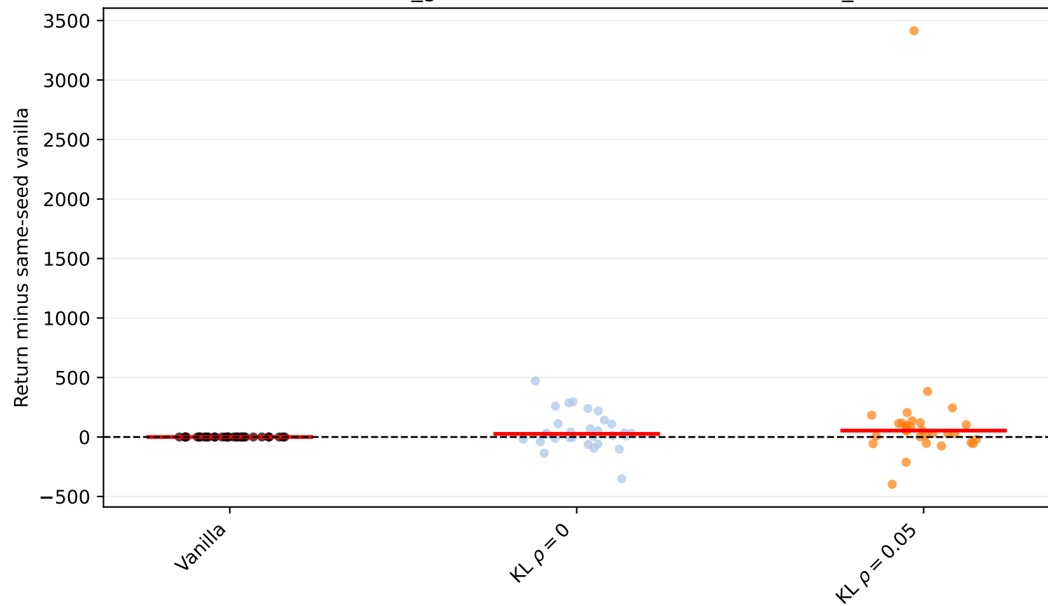
Walker2d-v5 actuator_gain factor=0.5: seed scatter (vanilla_subtracted)
