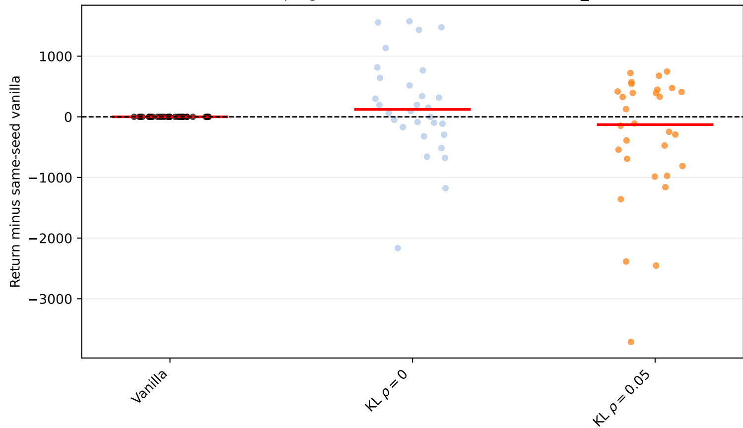
Walker2d-v5 damping factor=0.5: seed scatter (vanilla_subtracted)
