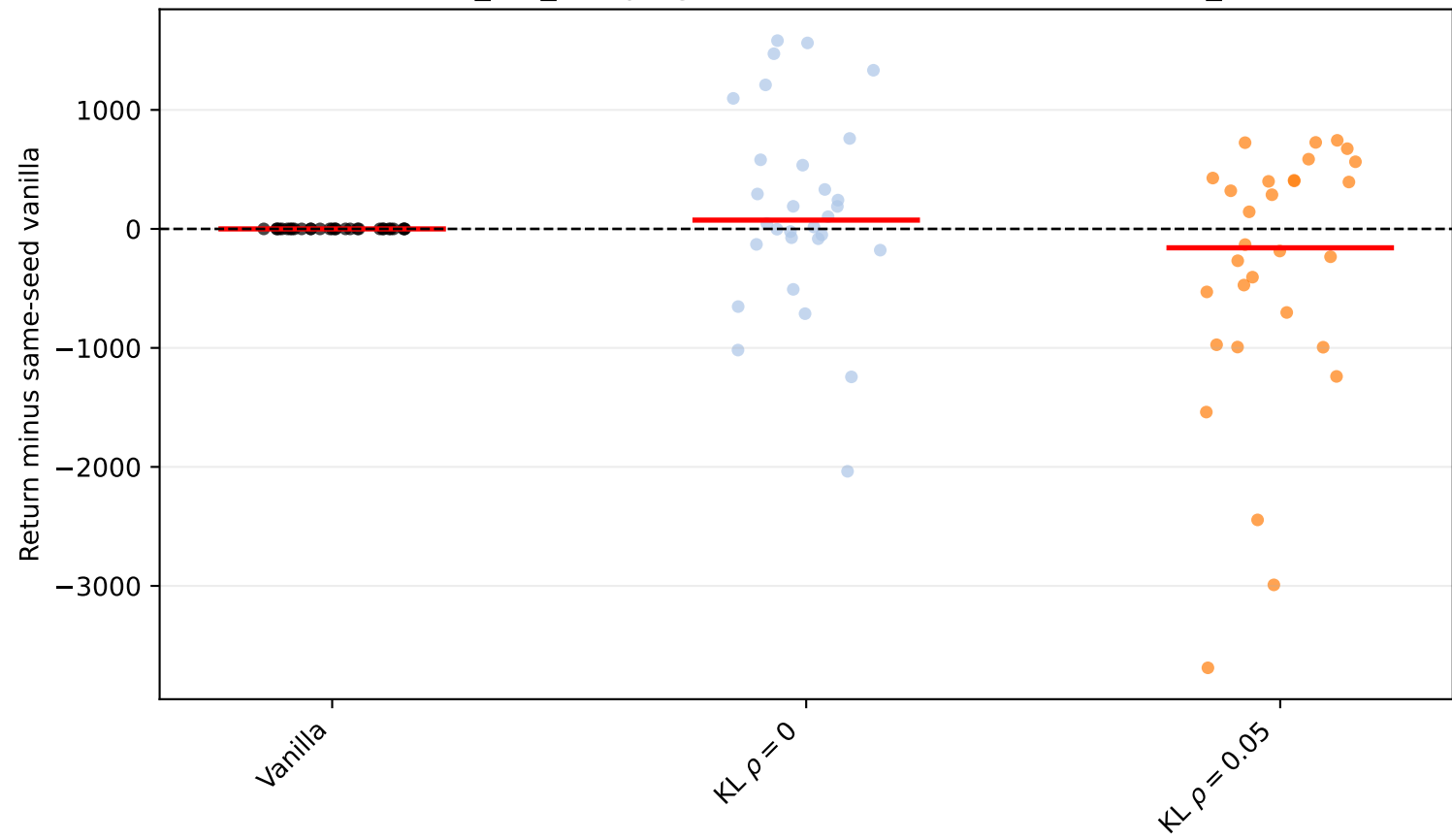
Walker2d-v5 foot_left_damping factor=0.5: seed scatter (vanilla_subtracted)
