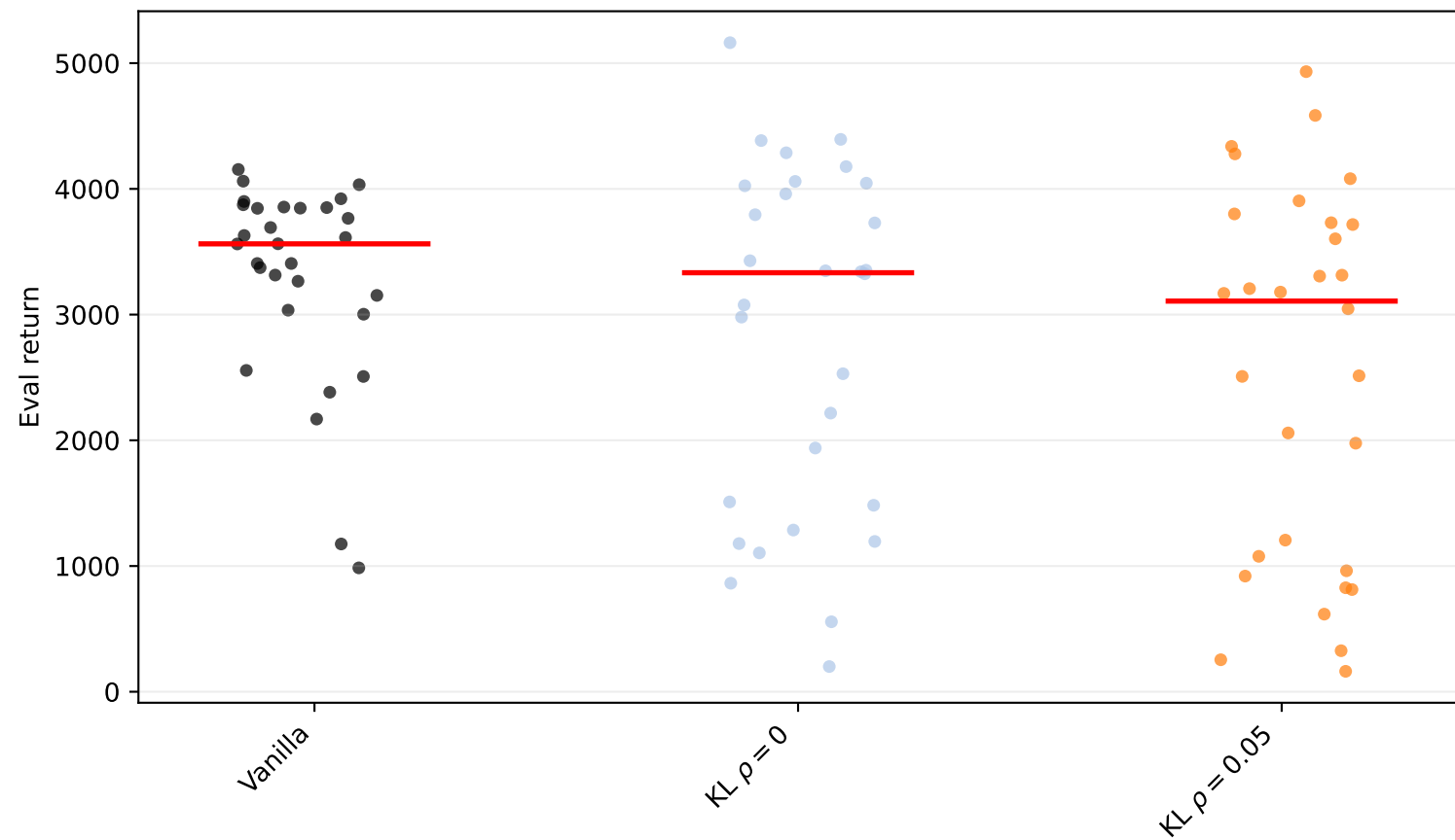
Walker2d-v5 friction factor=0.5: seed scatter (raw)
