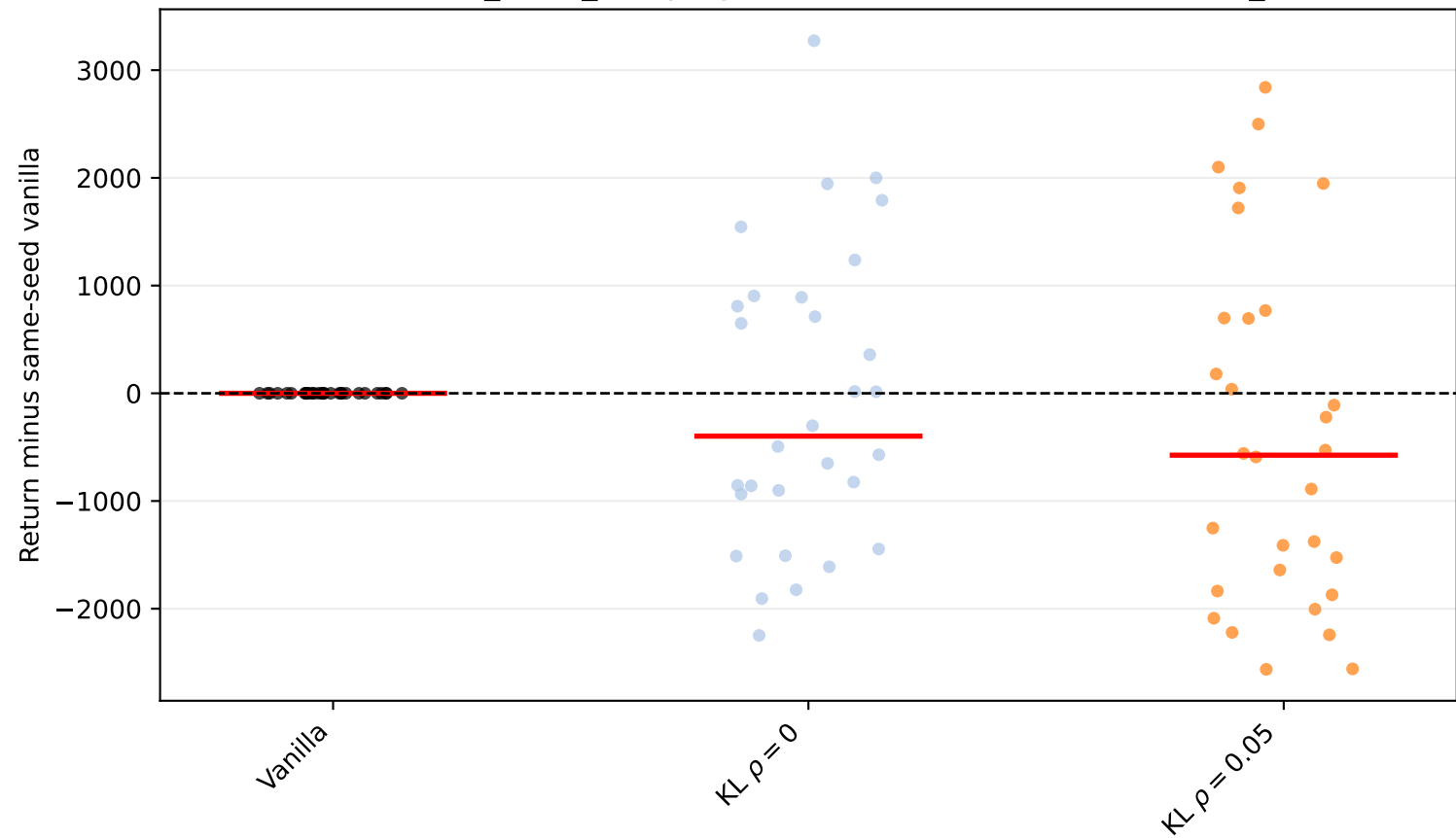
Walker2d-v5 friction_mass_damping factor=0.5: seed scatter (vanilla_subtracted)
