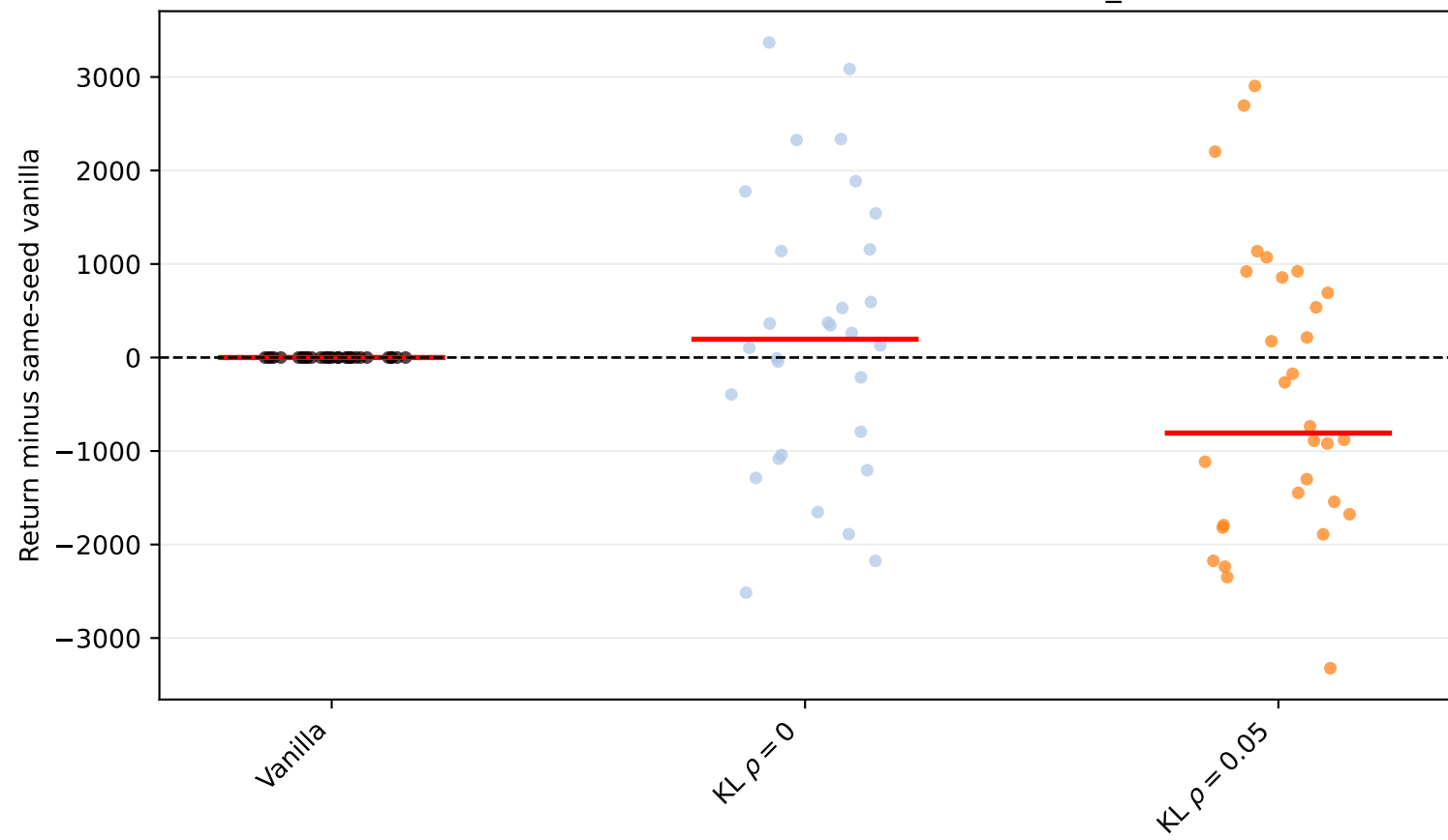
Walker2d-v5 mass factor=0.5: seed scatter (vanilla_subtracted)
