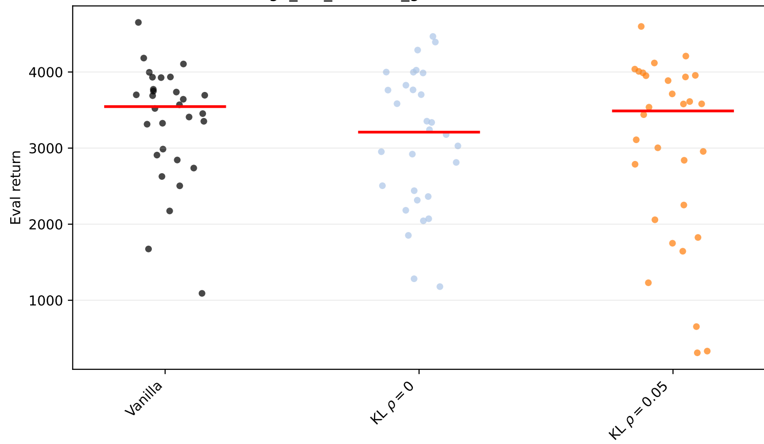
Walker2d-v5 thigh_left_actuator_gain factor=0.5: seed scatter (raw)
