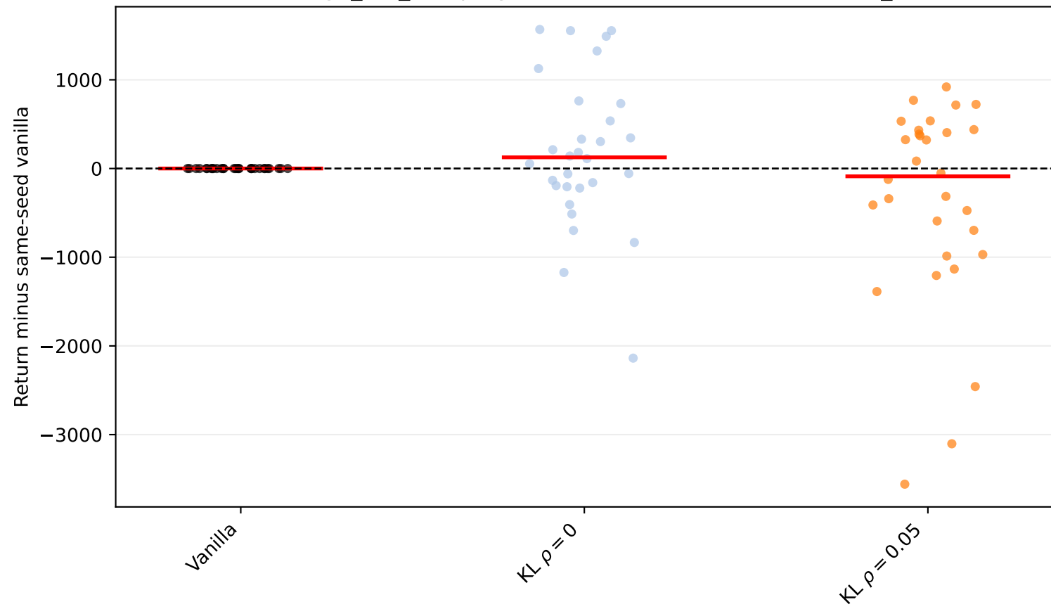
Walker2d-v5 thigh_left_damping factor=0.5: seed scatter (vanilla_subtracted)
