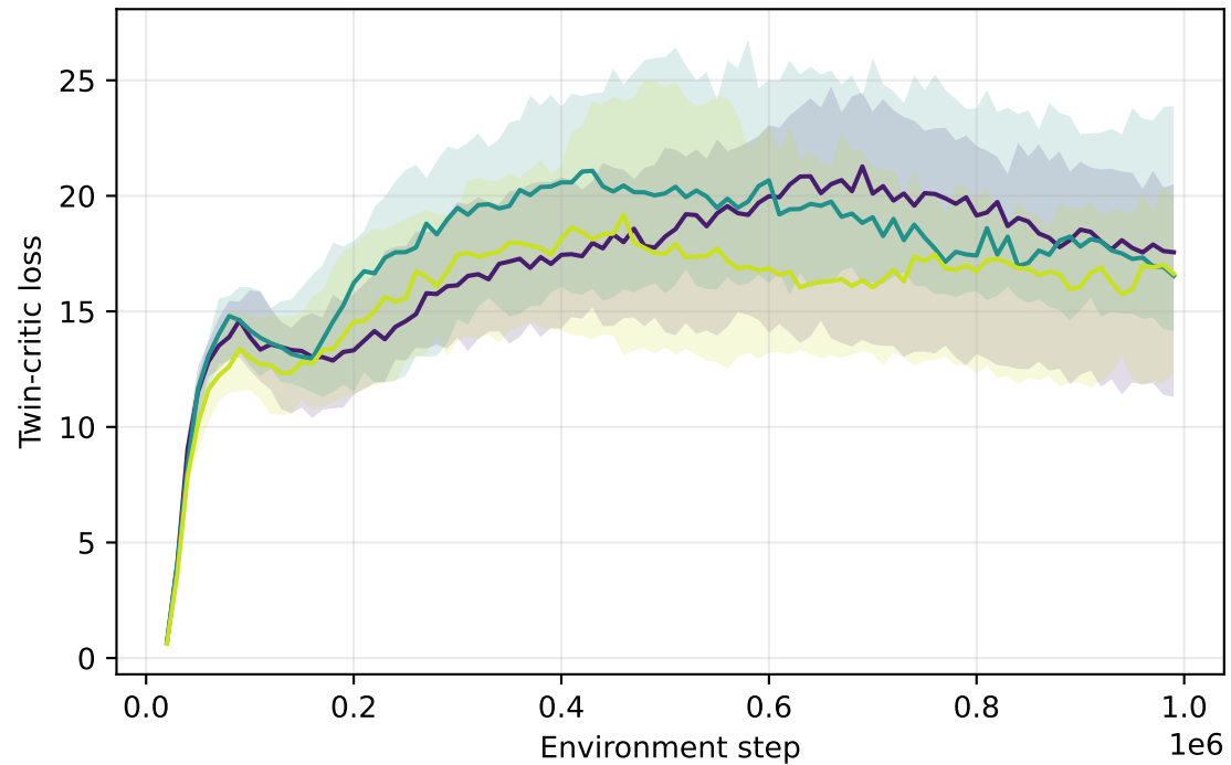
Physical-support TD3-KL: learning dynamics
