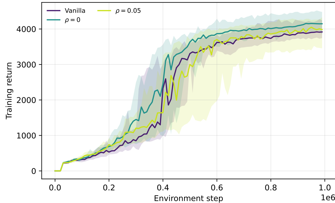
Physical-support TD3-KL: learning dynamics
