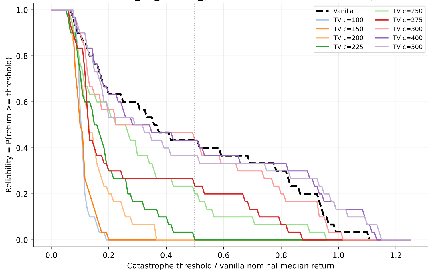
Walker2d-v5 foot_left_actuator_gain factor=0.5: robustness reliability curve
