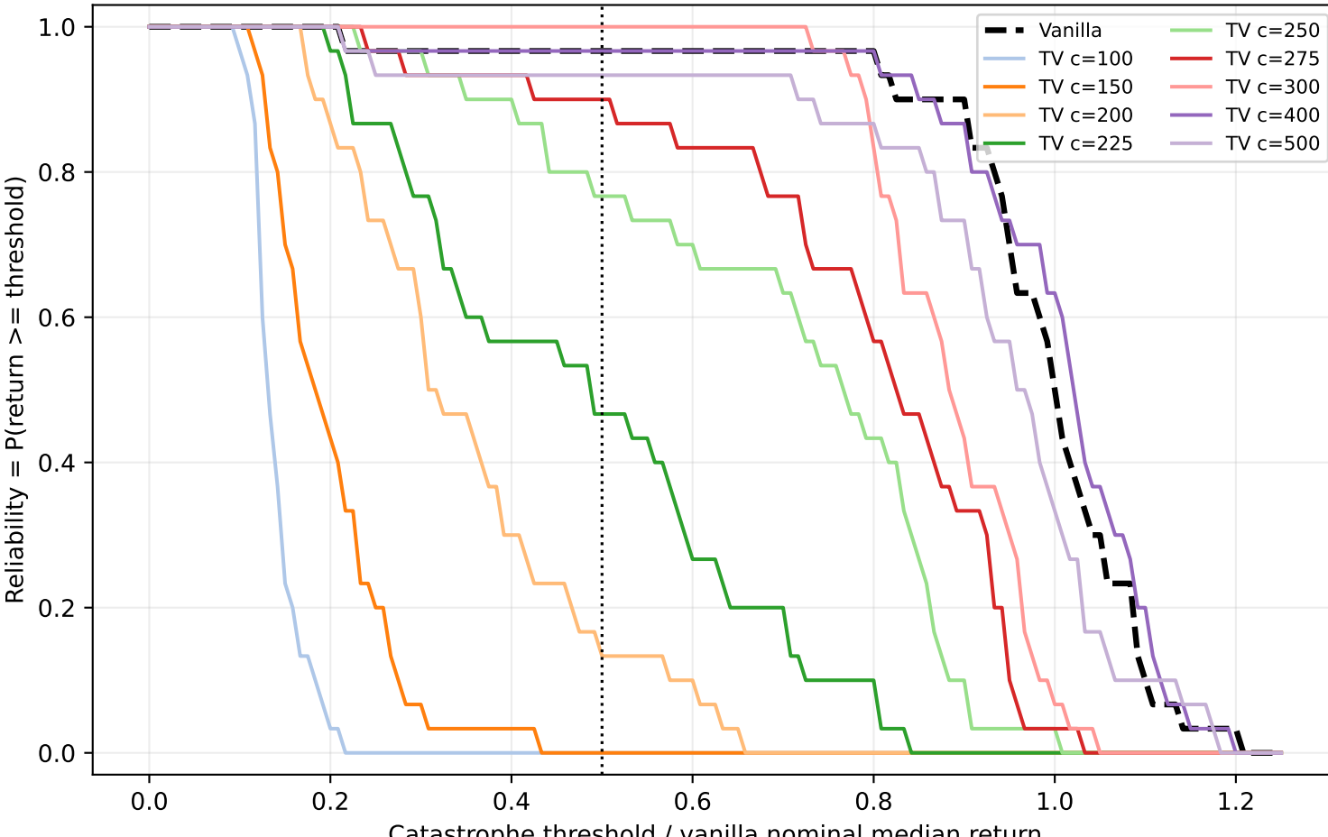
Walker2d-v5 foot left damping factor=0.5: robustness reliability curve
