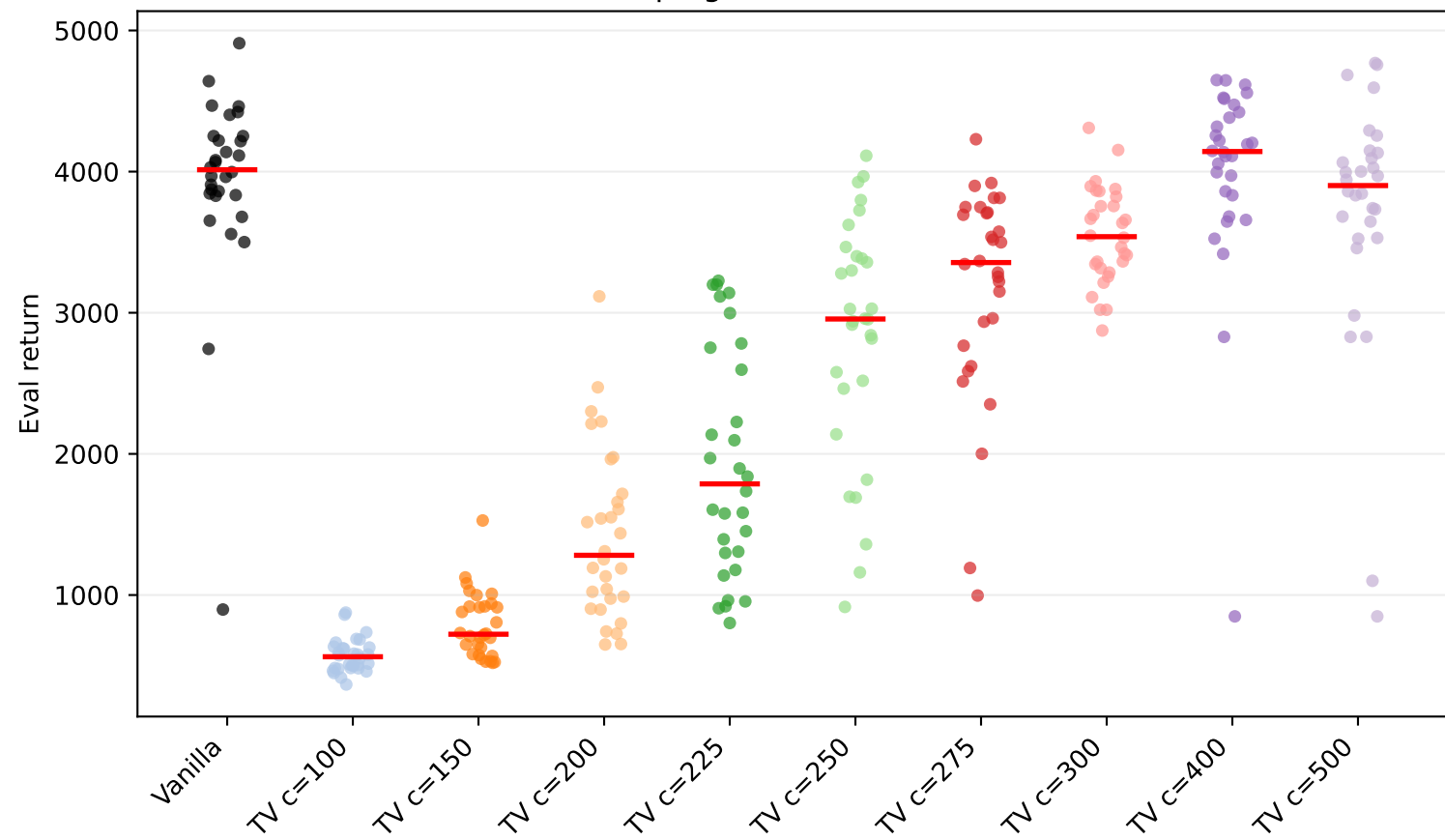
Walker2d-v5 damping factor=0.5: seed scatter (raw)
