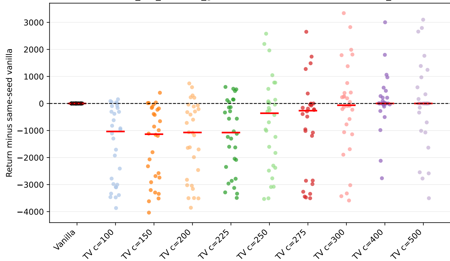
Walker2d-v5 foot_left_actuator_gain factor=0.5: seed scatter (vanilla_subtracted)
