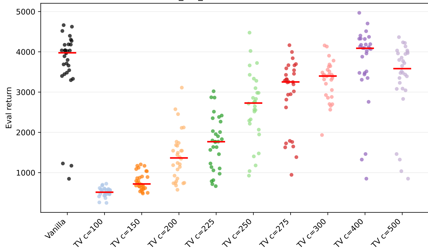
Walker2d-v5 foot_left_mass factor=0.5: seed scatter (raw)
