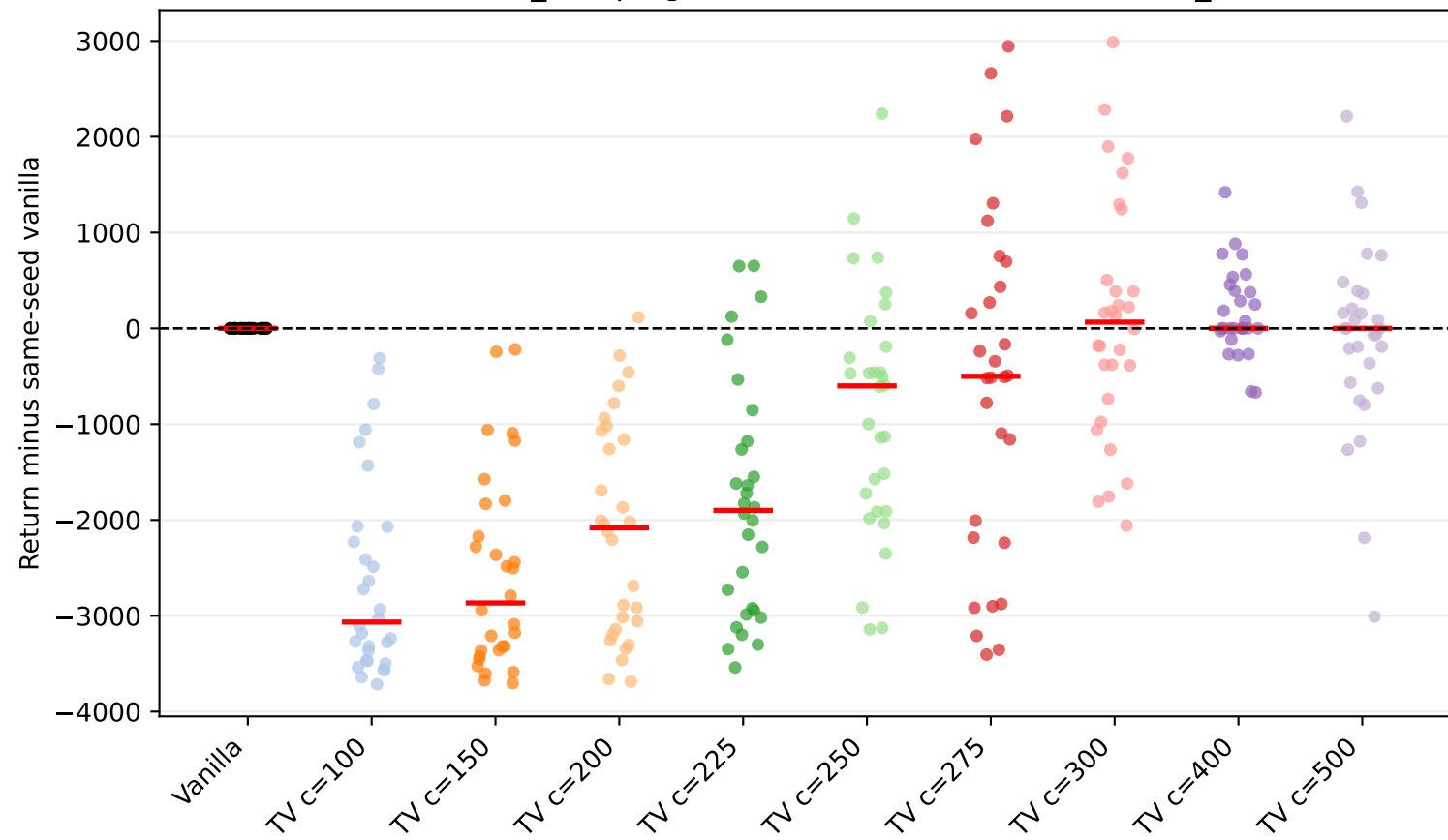
Walker2d-v5 friction_damping factor=0.5: seed scatter (vanilla_subtracted)
