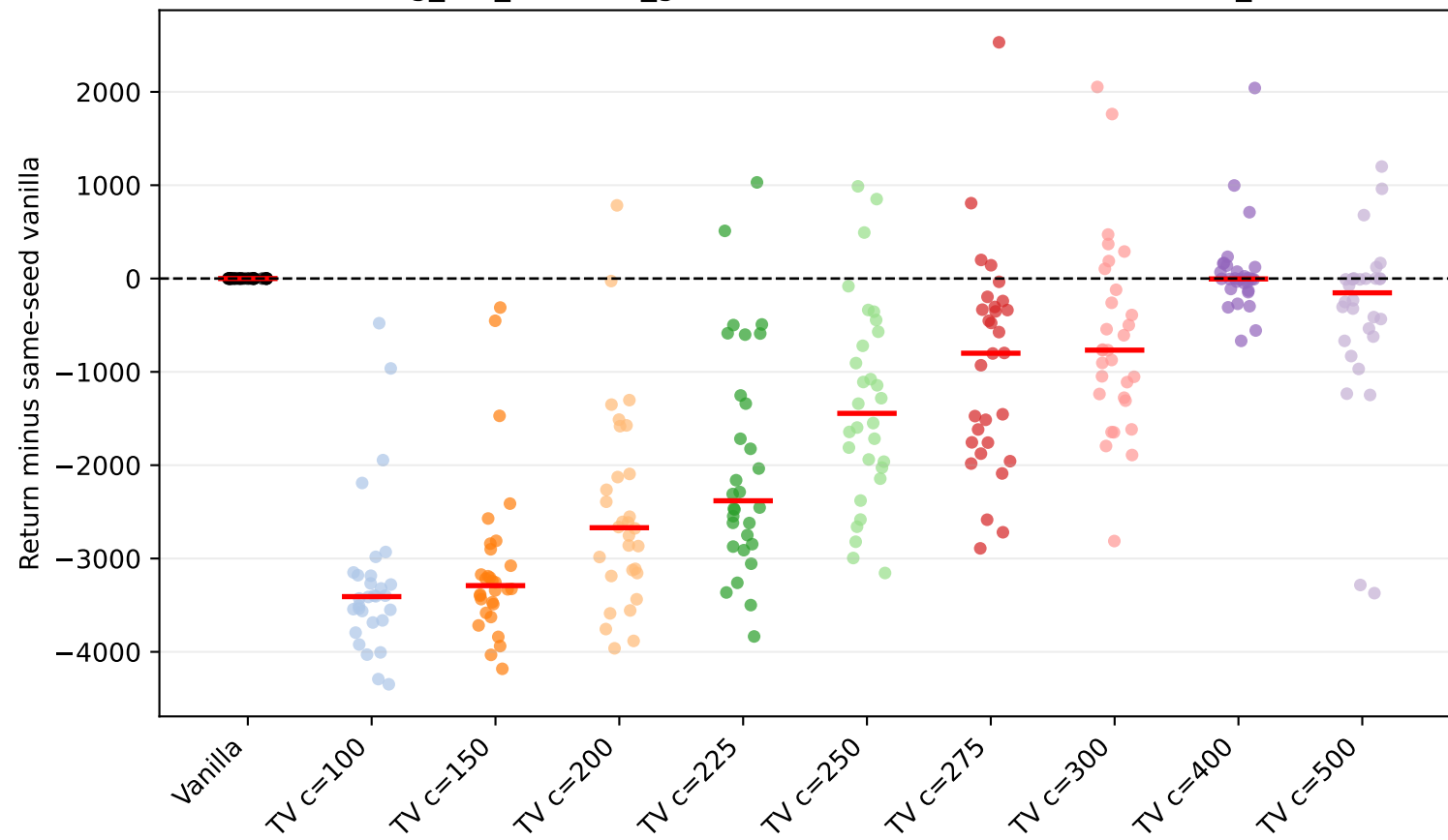
Walker2d-v5 leg_left_actuator_gain factor=0.5: seed scatter (vanilla_subtracted)
