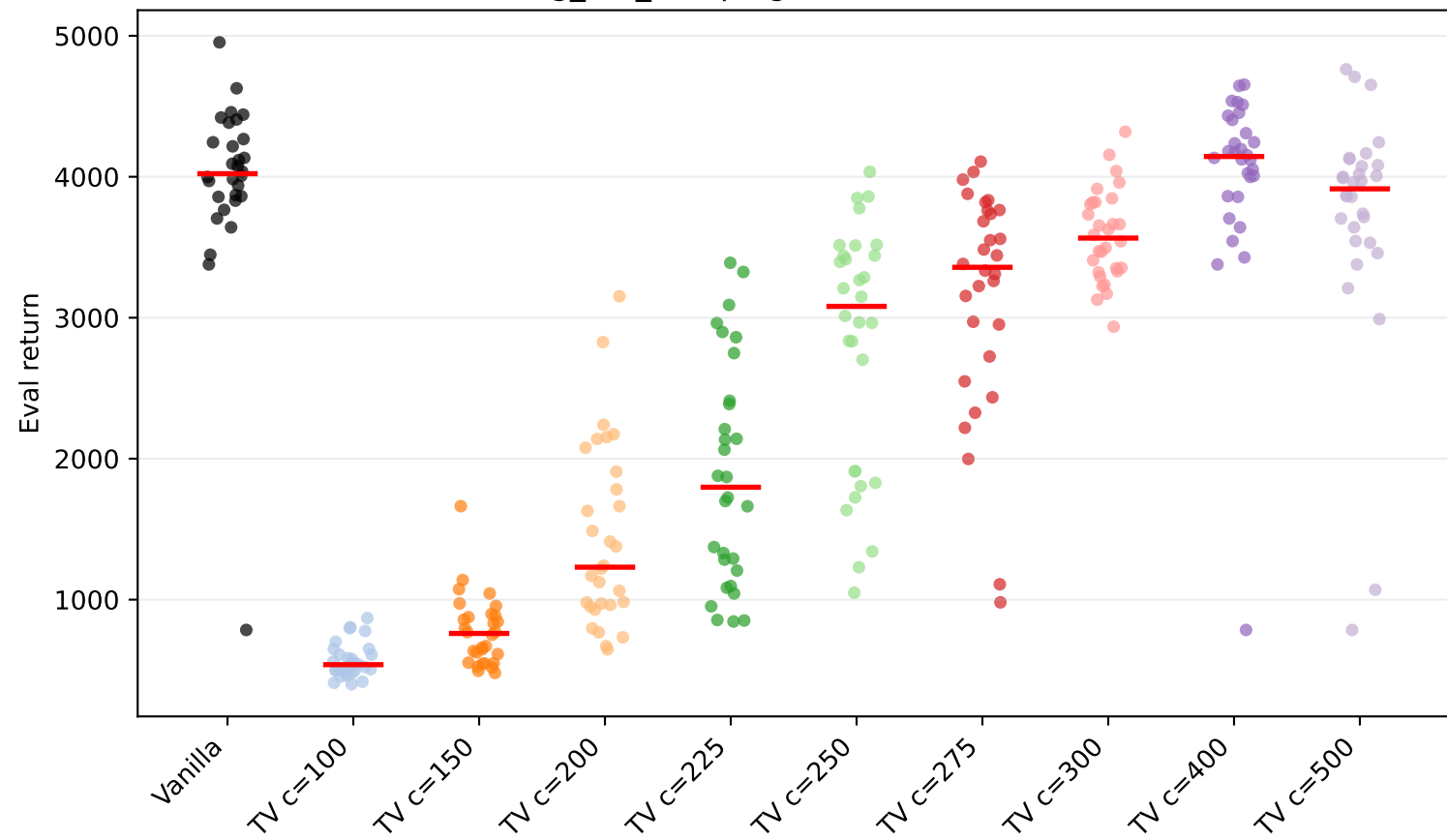
Walker2d-v5 leg_left_damping factor=0.5: seed scatter (raw)
