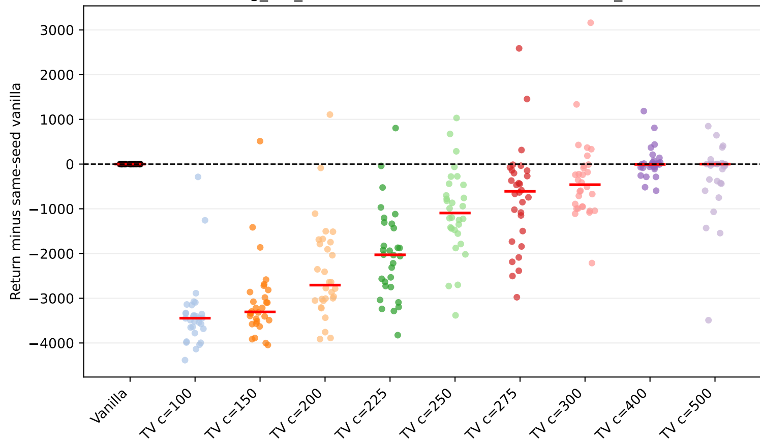
Walker2d-v5 leg_left_mass factor=0.5: seed scatter (vanilla_subtracted)
