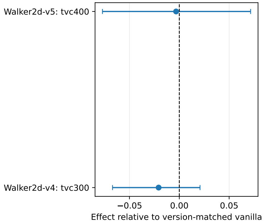
Catastrophe probability
