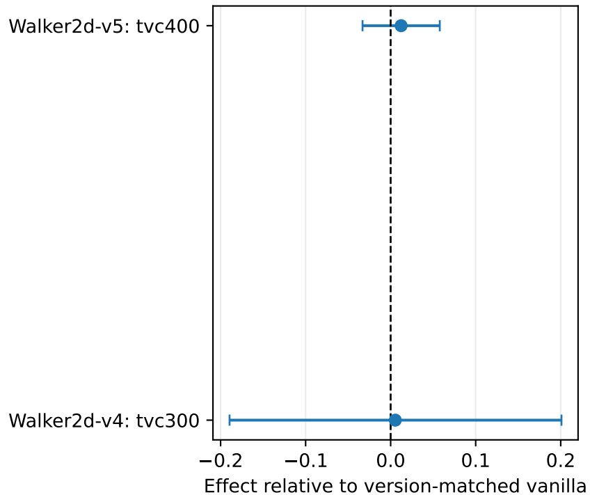
Axis-balanced CVaR20
