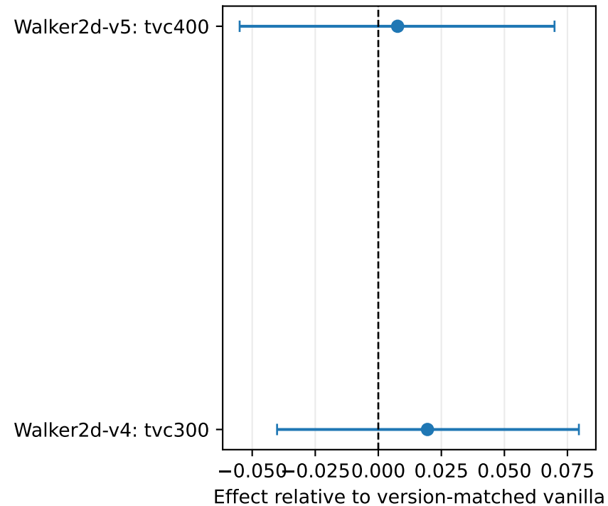
Reliability AUC
