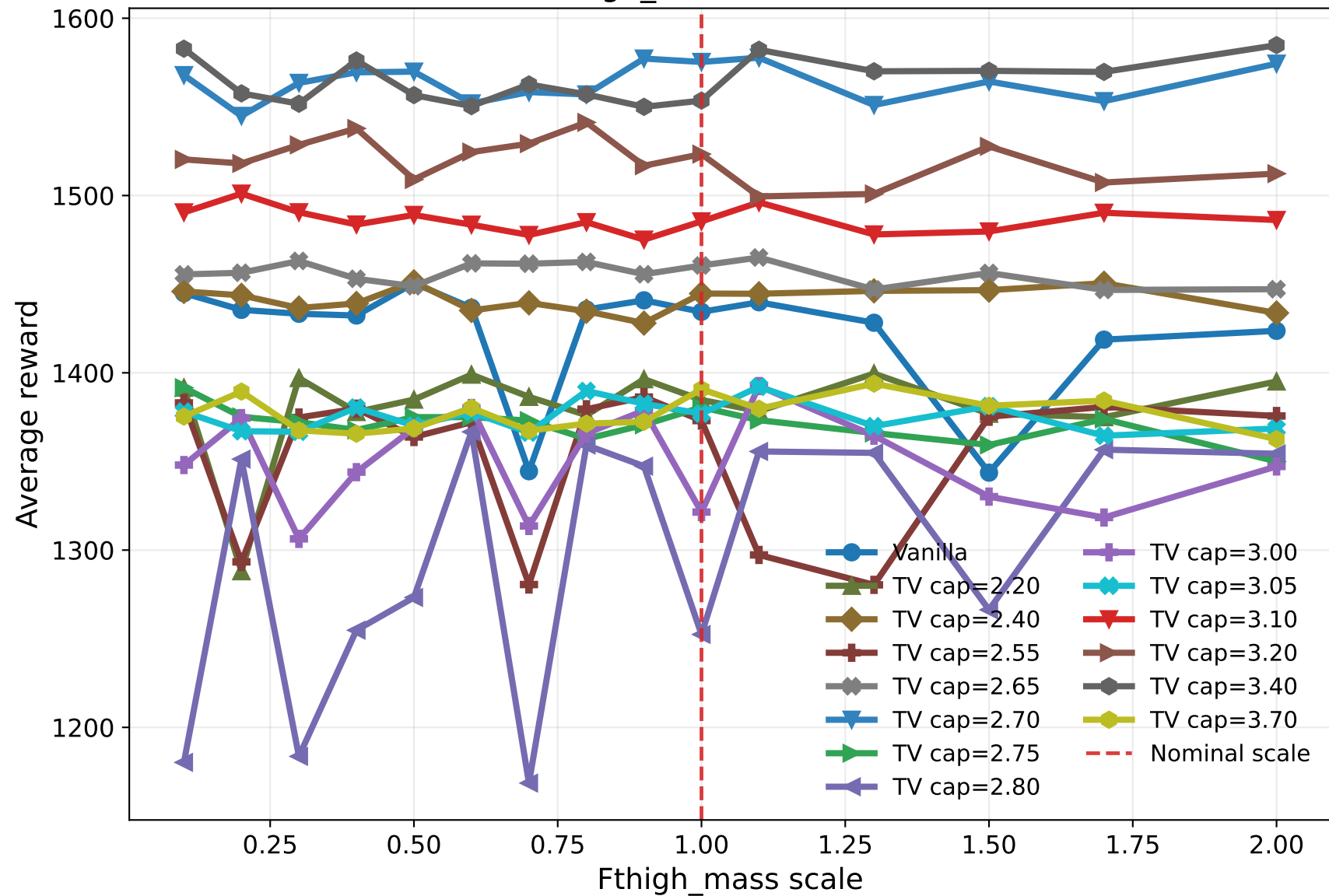
Fthigh_mass robustness
