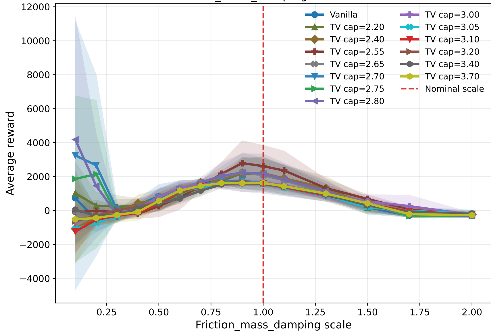
Friction_mass_damping robustness
