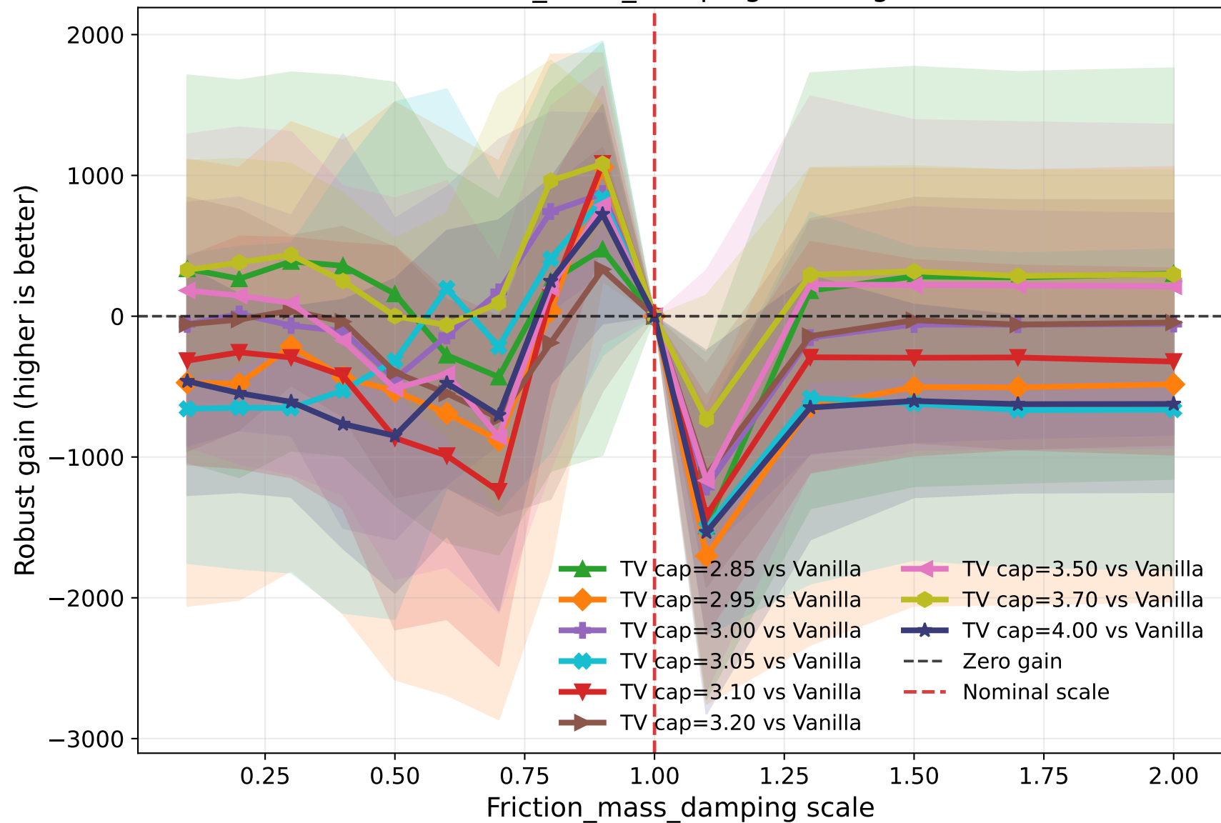
Friction_mass_damping robust gain
