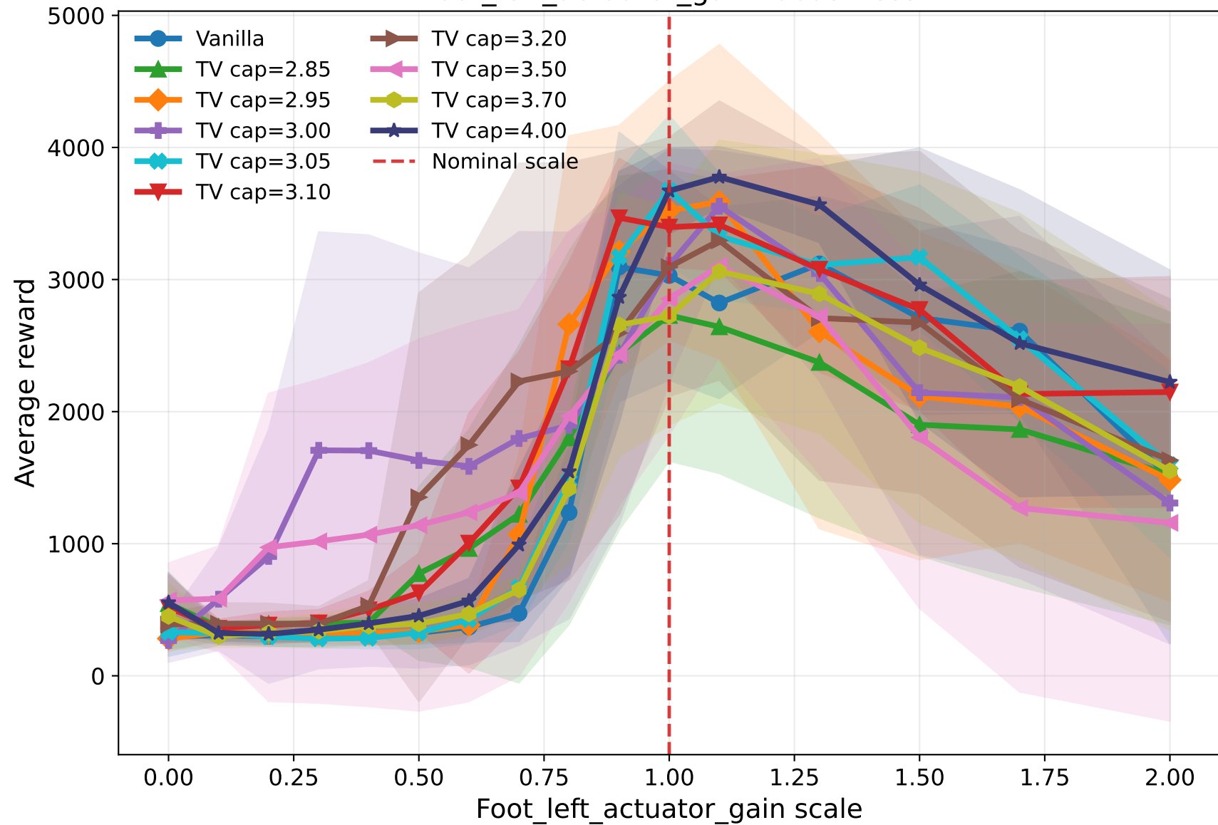
Foot_left_actuator_gain robustness
