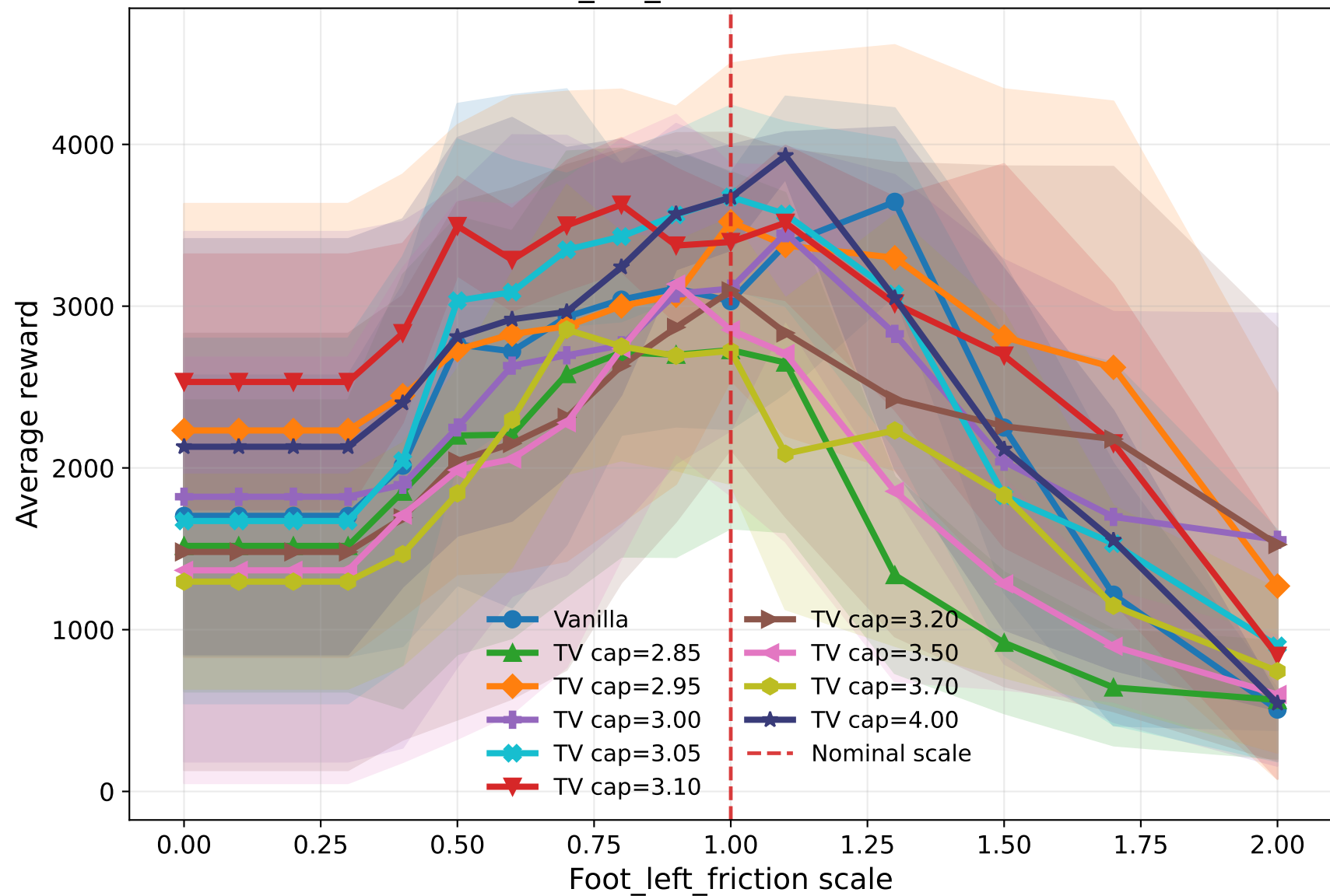
Foot_left_friction robustness
