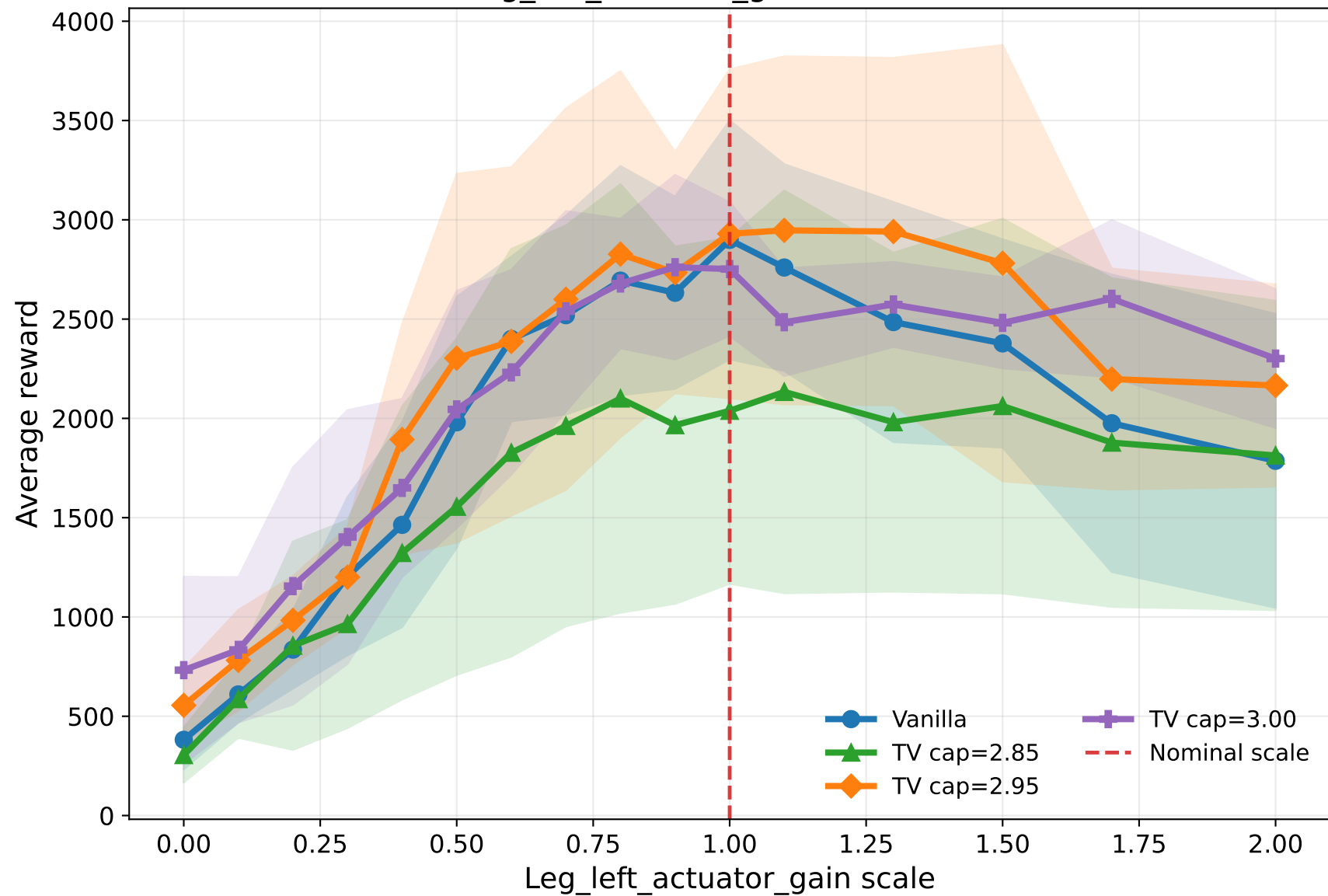
Leg_left_actuator_gain robustness
