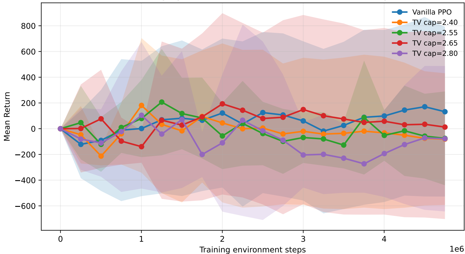
HalfCheetah PPO Learning Dynamics Under Actuator Gain Perturbation (gain scale = 0.5)
