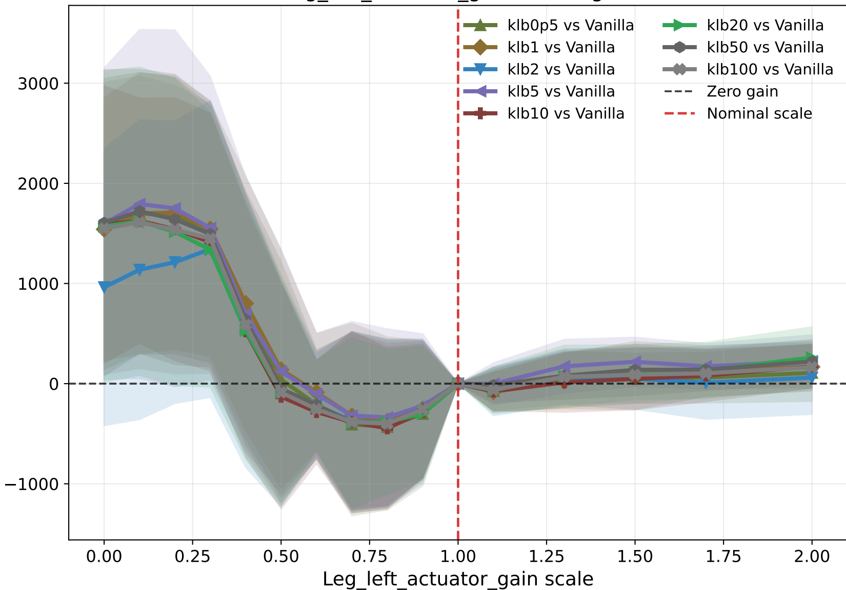
Leg_left_actuator_gain robust gain
