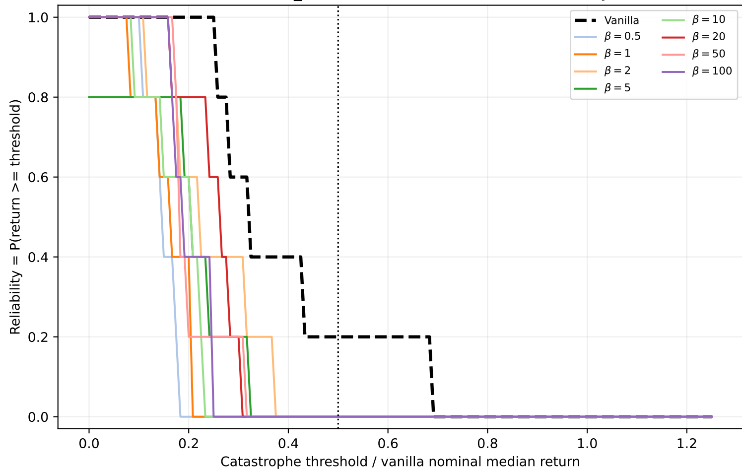
Walker2d-v4 action noise factor=0.5: robustness reliability curve
