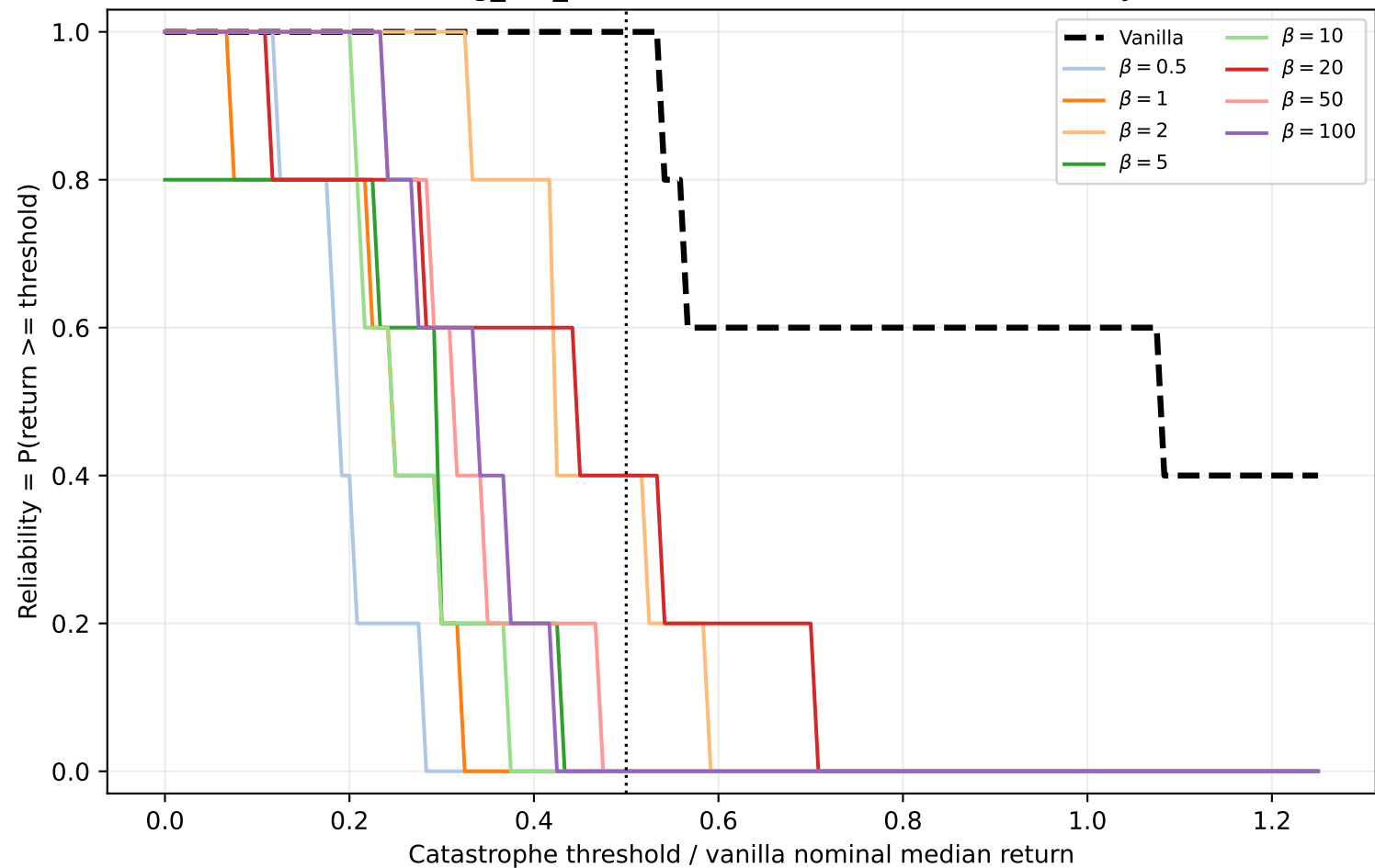
Walker2d-v4 leg left mass factor=0.5: robustness reliability curve
