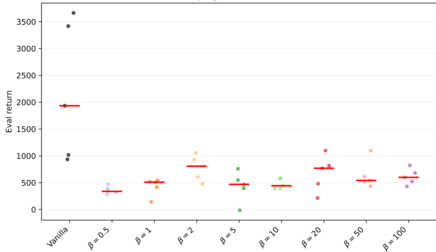
Walker2d-v4 damping factor=0.5: seed scatter (raw)
