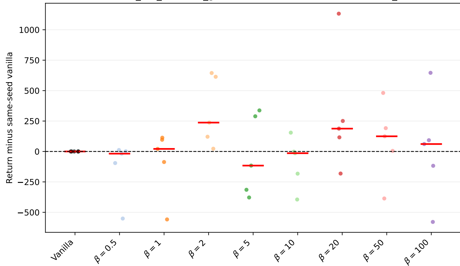
Walker2d-v4 foot_left_actuator_gain factor=0.5: seed scatter (vanilla_subtracted)
