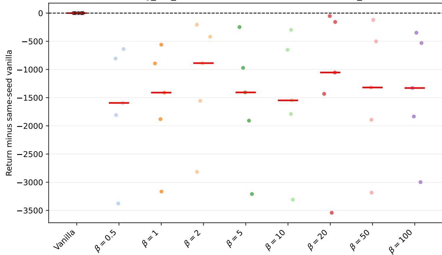
Walker2d-v4 leg_left_mass factor=0.5: seed scatter (vanilla_subtracted)
