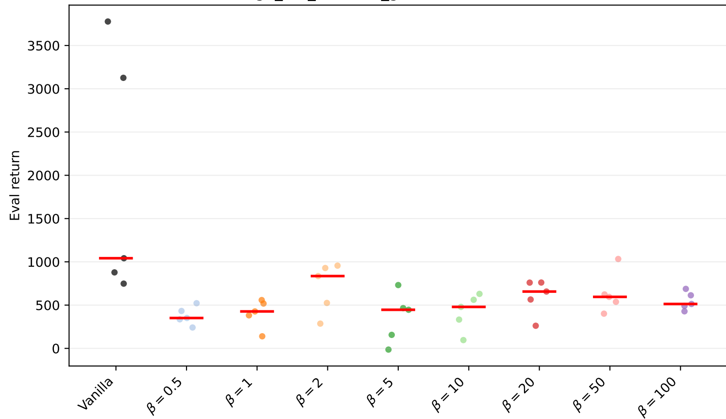
Walker2d-v4 thigh_left_actuator_gain factor=0.5: seed scatter (raw)
