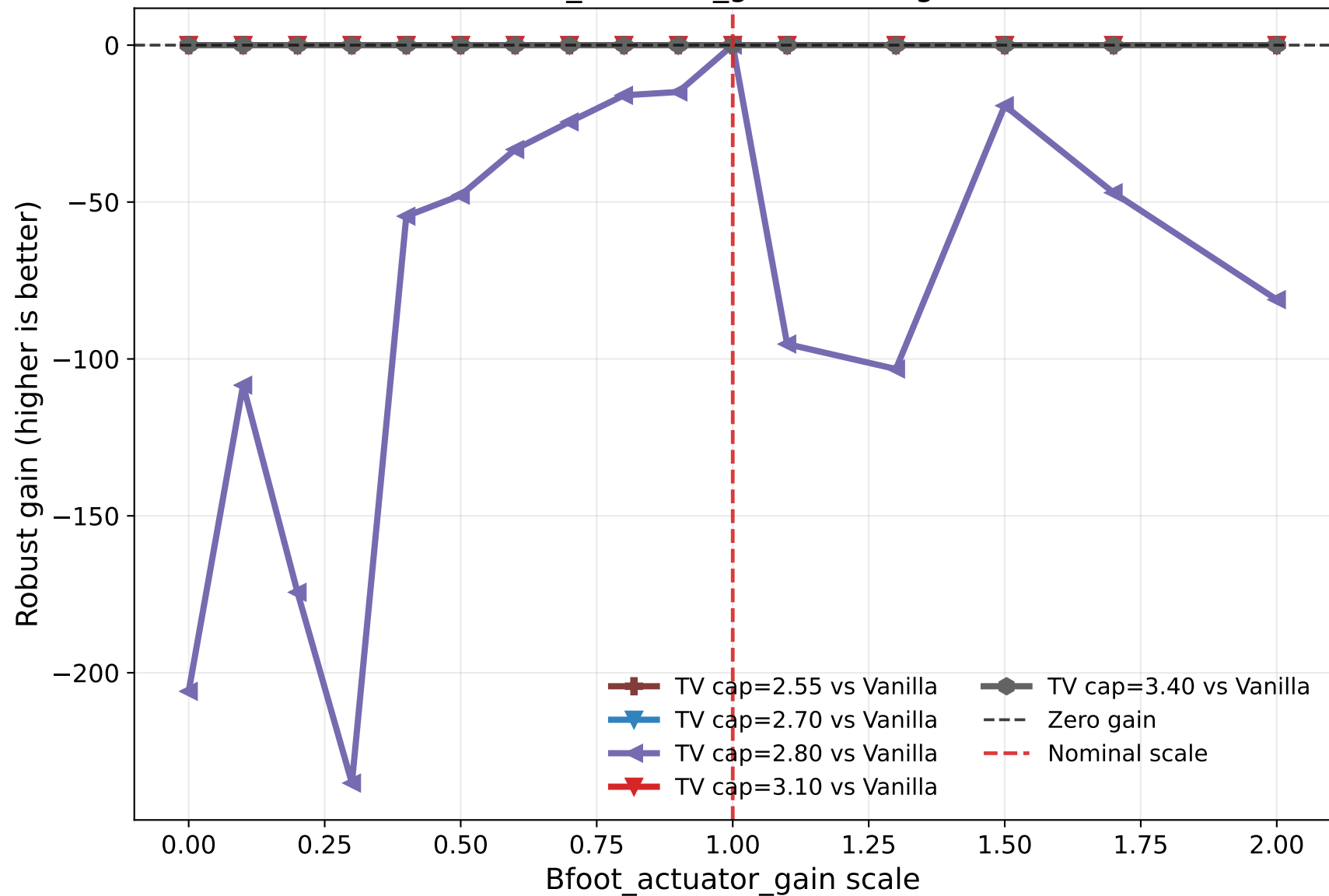
Bfoot_actuator_gain robust gain
