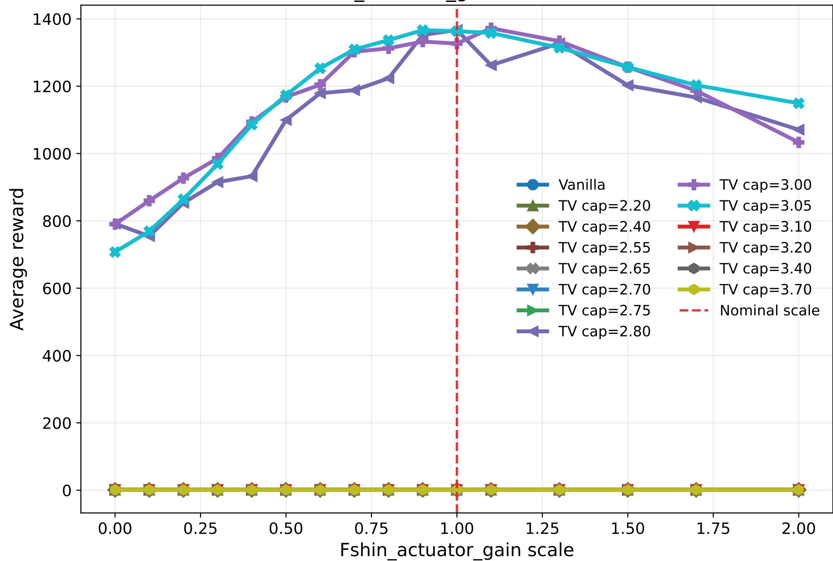
Fshin_actuator_gain robustness
