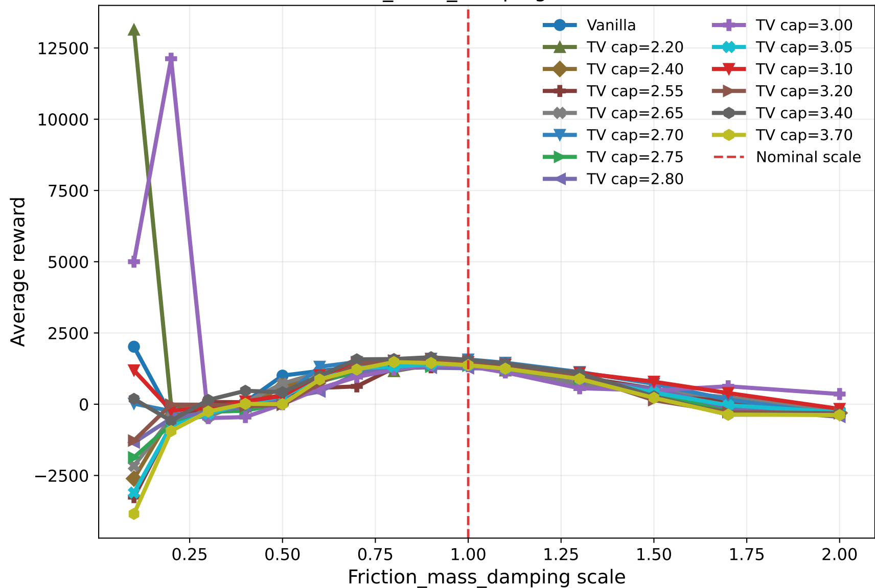
Friction_mass_damping robustness
