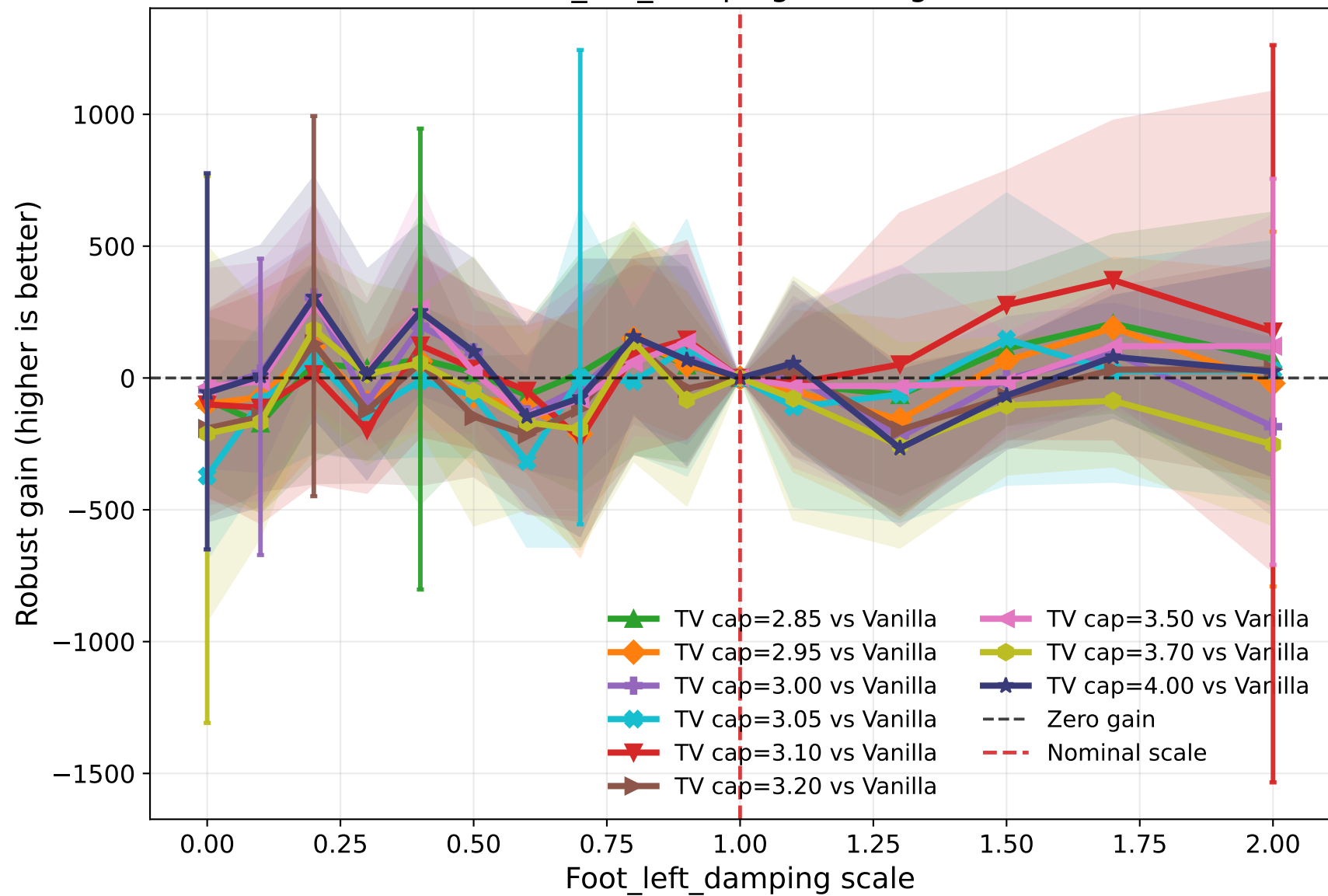
Foot_left_damping robust gain
