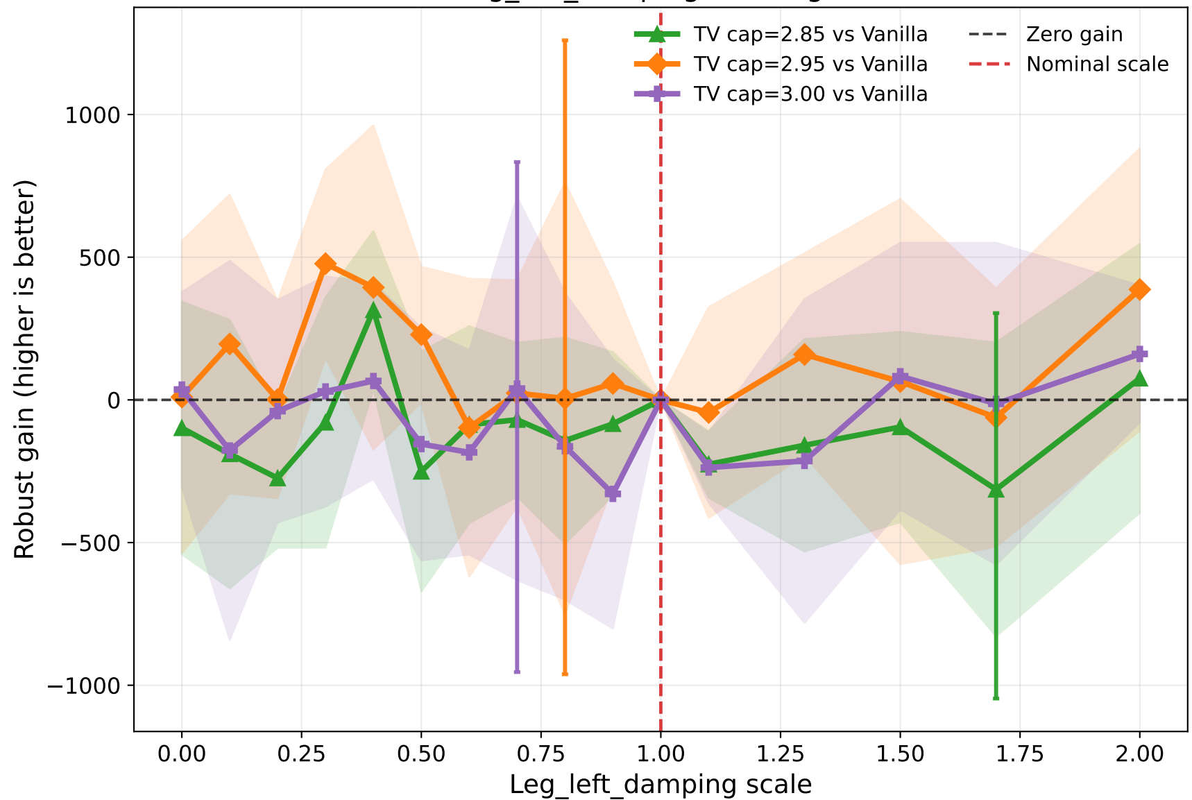
Leg_left_damping robust gain
