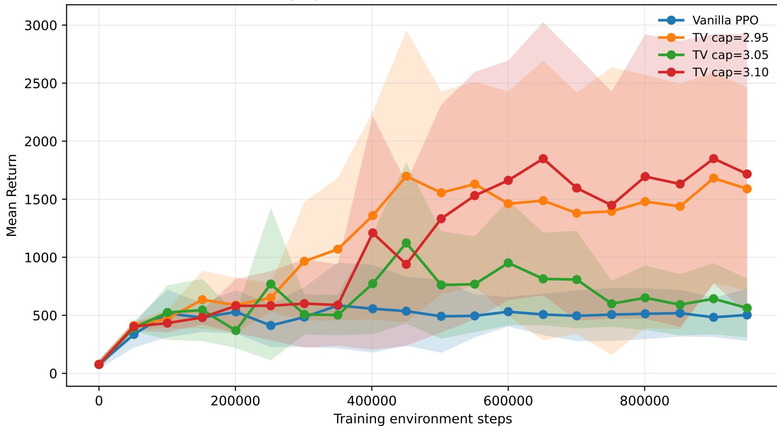
Walker2d PPO Learning Dynamics Under Mass Perturbation (mass scale = 0.5)
