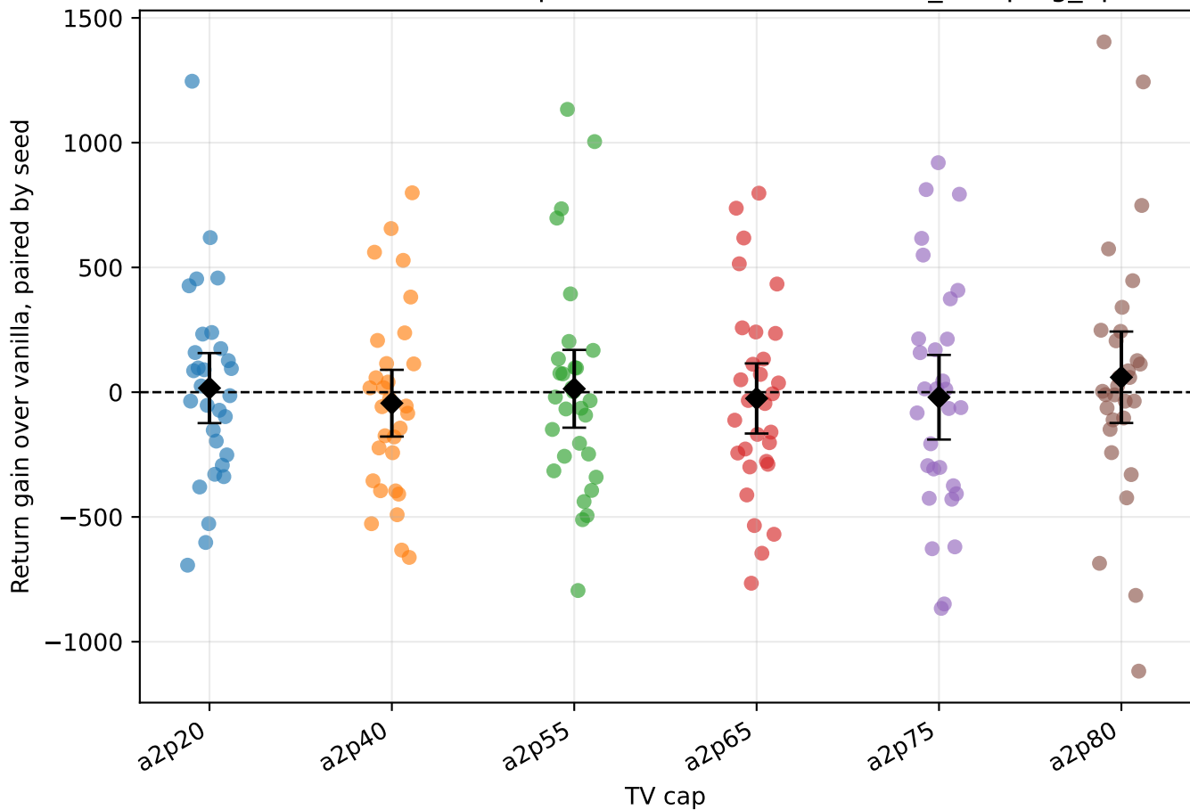
HalfCheetah 30-seed expanded confirmation: mass_damping_0p5
