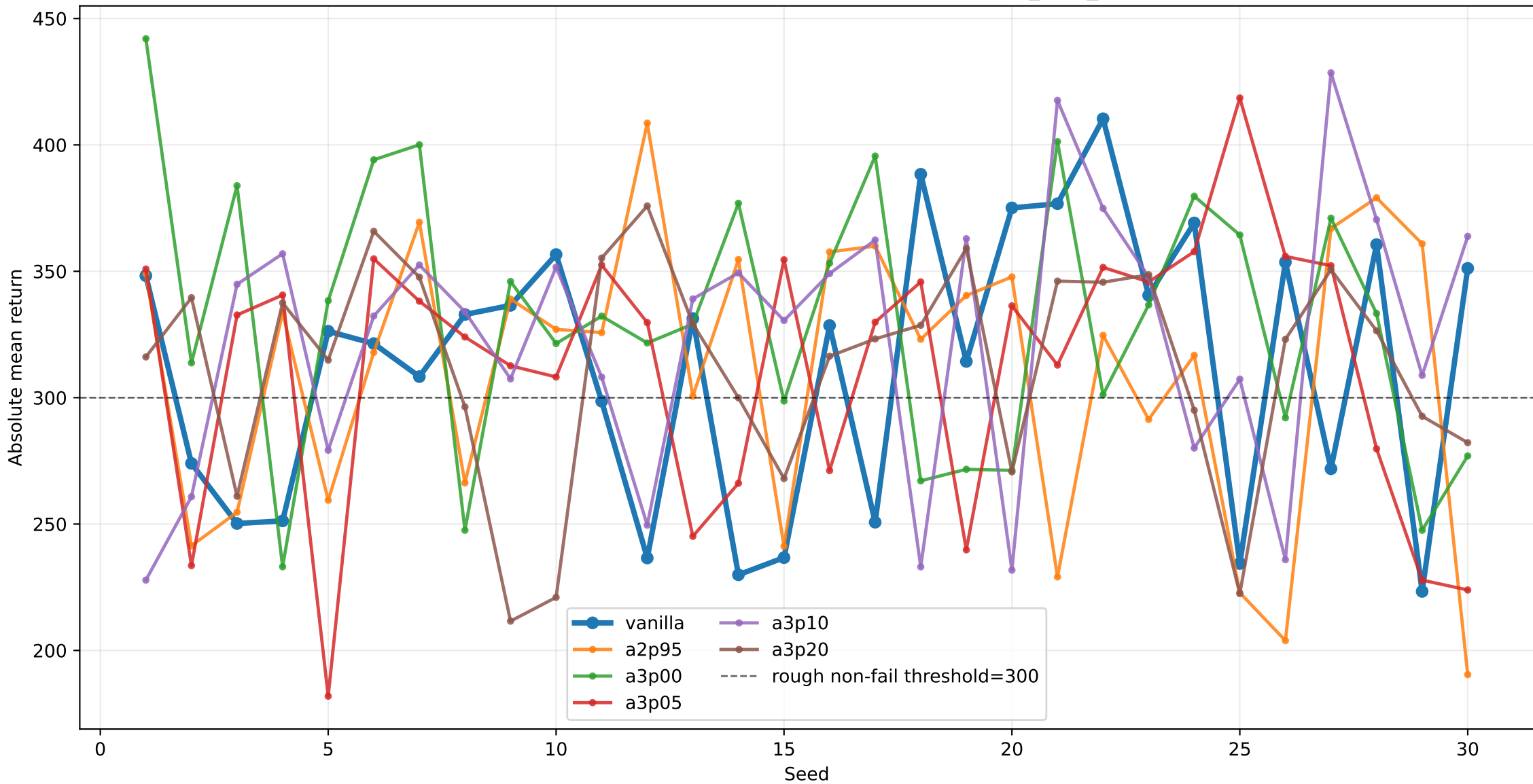
Walker2d: absolute returns by seed under actuator_gain_0p5
