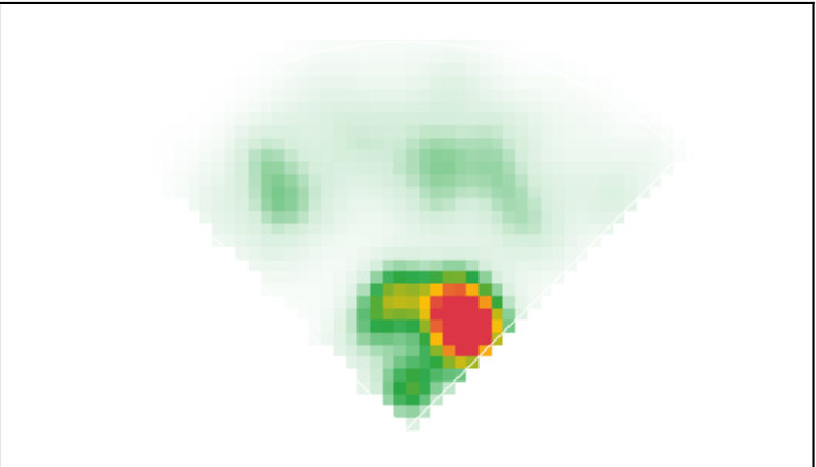
Inpainted (k=50)
