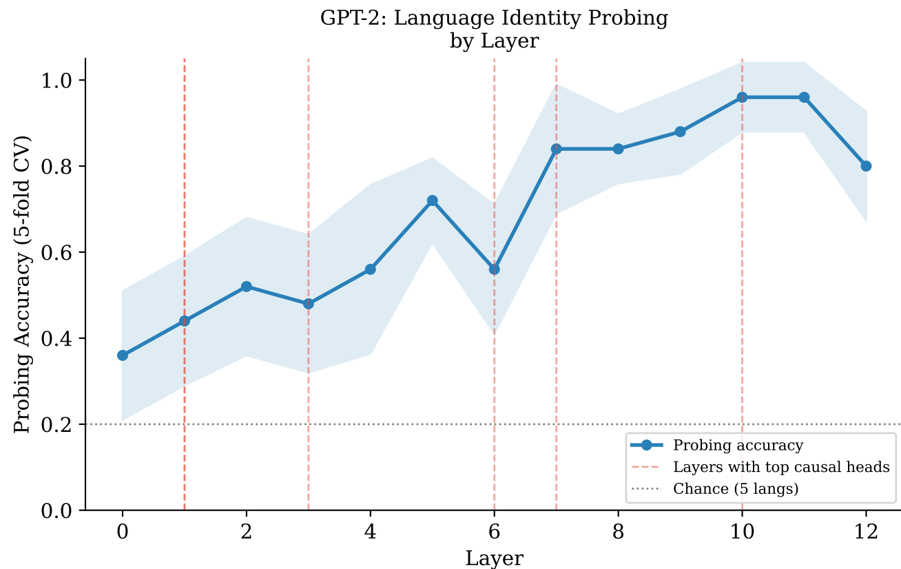
Linear Probe Accuracy for Language Identity Prediction by Layer Red dashed lines mark layers containing top causal heads from ablation sweep
