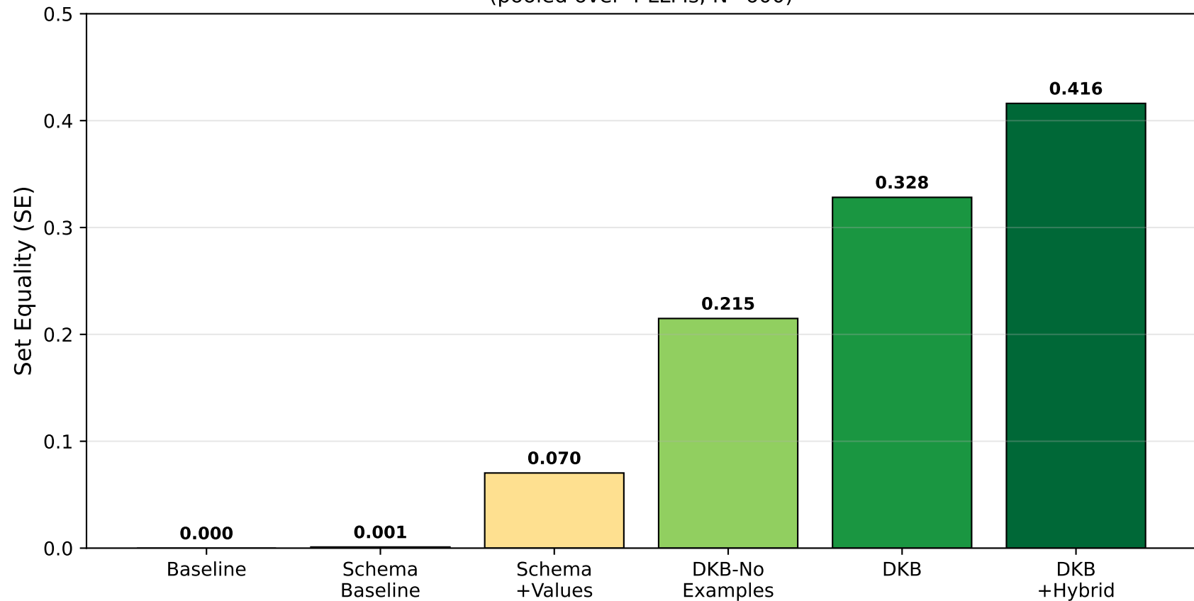
Ablation: Component Contribution to SE (pooled over 4 LLMs, N=600)
