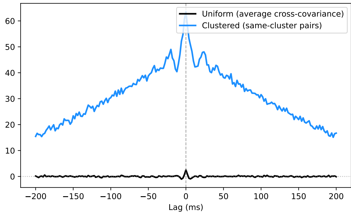
Cross-covariance
