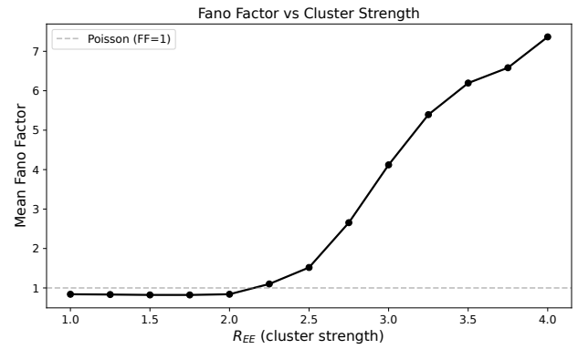
Figure 8. Mean Fano factor as a function of cluster strength ( R_{EE} ). As within-cluster connection strength increases, the network transitions from Poisson-like variability to super-Poisson variability. The dashed line indicates the Poisson baseline (FF = 1).
