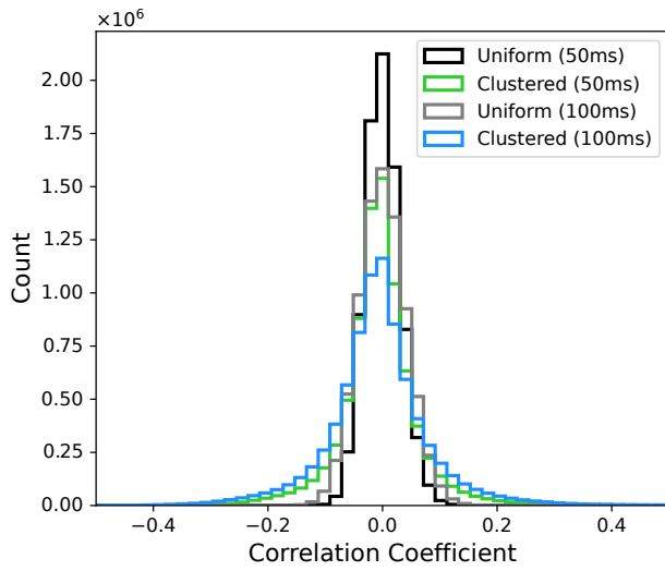
Figure 6. Distribution of pairwise spike count correlations for all neuron pairs. Correlations remain centered near zero on average for both network types.
