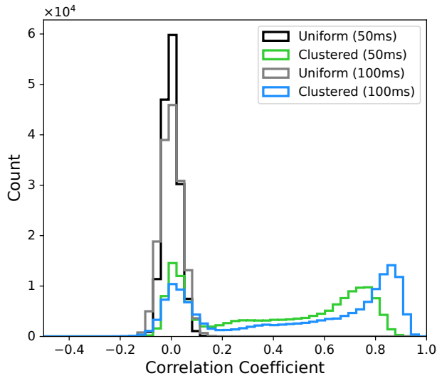
Figure 7. Distribution of pairwise spike count correlations for within-cluster pairs only. The clustered network shows a heavy positive tail that increases with counting window size (50 ms vs. 100 ms).
