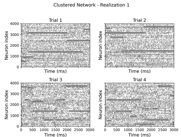
Figure 2. Spike rasters from a clustered network across multiple trials.
