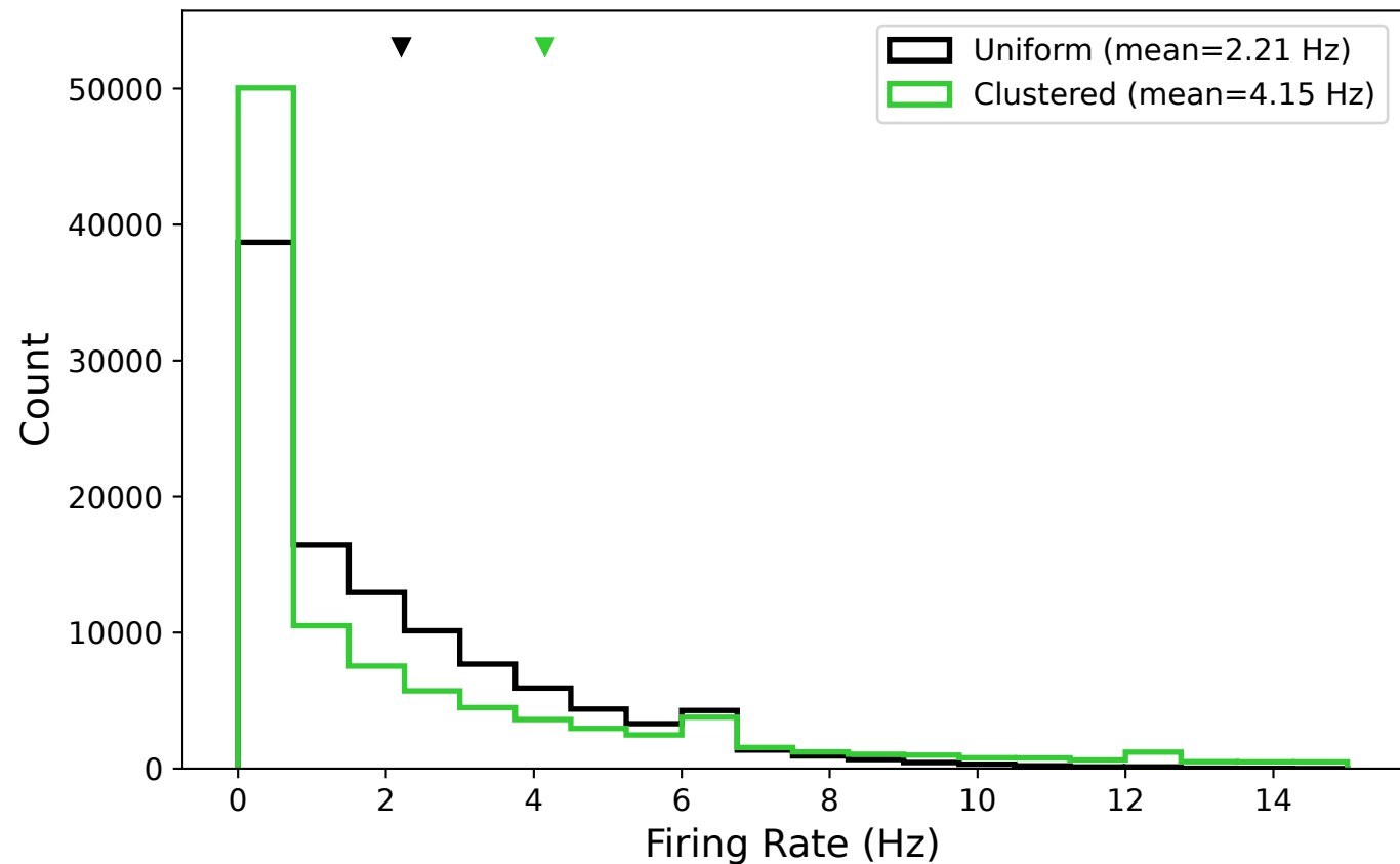
Firing Rate Distribution (Excitatory Neurons) 3 realizations x 9 trials
