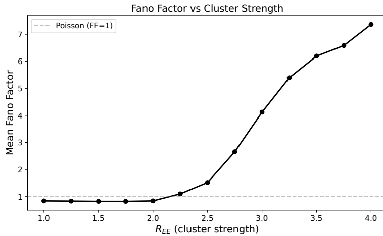
Figure 5. Mean Fano factor as a function of cluster strength ( R_{EE} ). As within-cluster connection strength increases, the network transitions from Poisson-like variability to super-Poisson variability.
