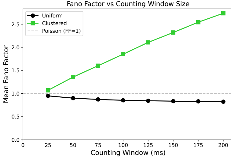
Figure 2. Mean Fano factor as a function of counting window size. In the clustered network, the Fano factor increases with window size, reflecting slow rate fluctuations. The uniform network remains near the Poisson baseline ( FF = 1 ).
