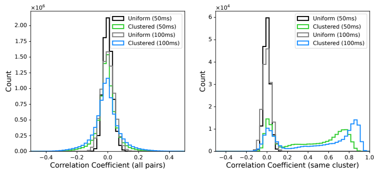
Figure 3. Distribution of pairwise spike count correlations for all neuron pairs (left) and within-cluster pairs only (right). While correlations remain centered near zero on average, within-cluster pairs in the clustered network show a heavy positive tail that increases with counting window size (50 ms vs. 100 ms).
