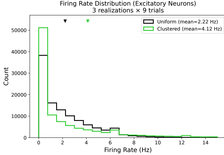
Figure 4. Distribution of firing rates for excitatory neurons in uniform and clustered networks. Both networks maintain low mean firing rates, though the clustered network shows a broader distribution reflecting the alternation between high and low activity states.
