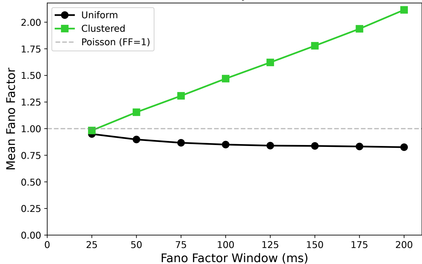
Fano Factor vs Analysis Window Size
